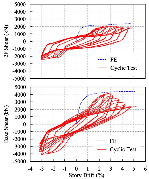
Fig. 9. Monotonic pushover curves and hystereses of Phase II cyclic test
