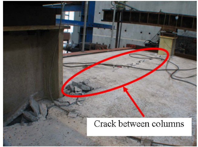
Fig. 12. Crack at top slab
