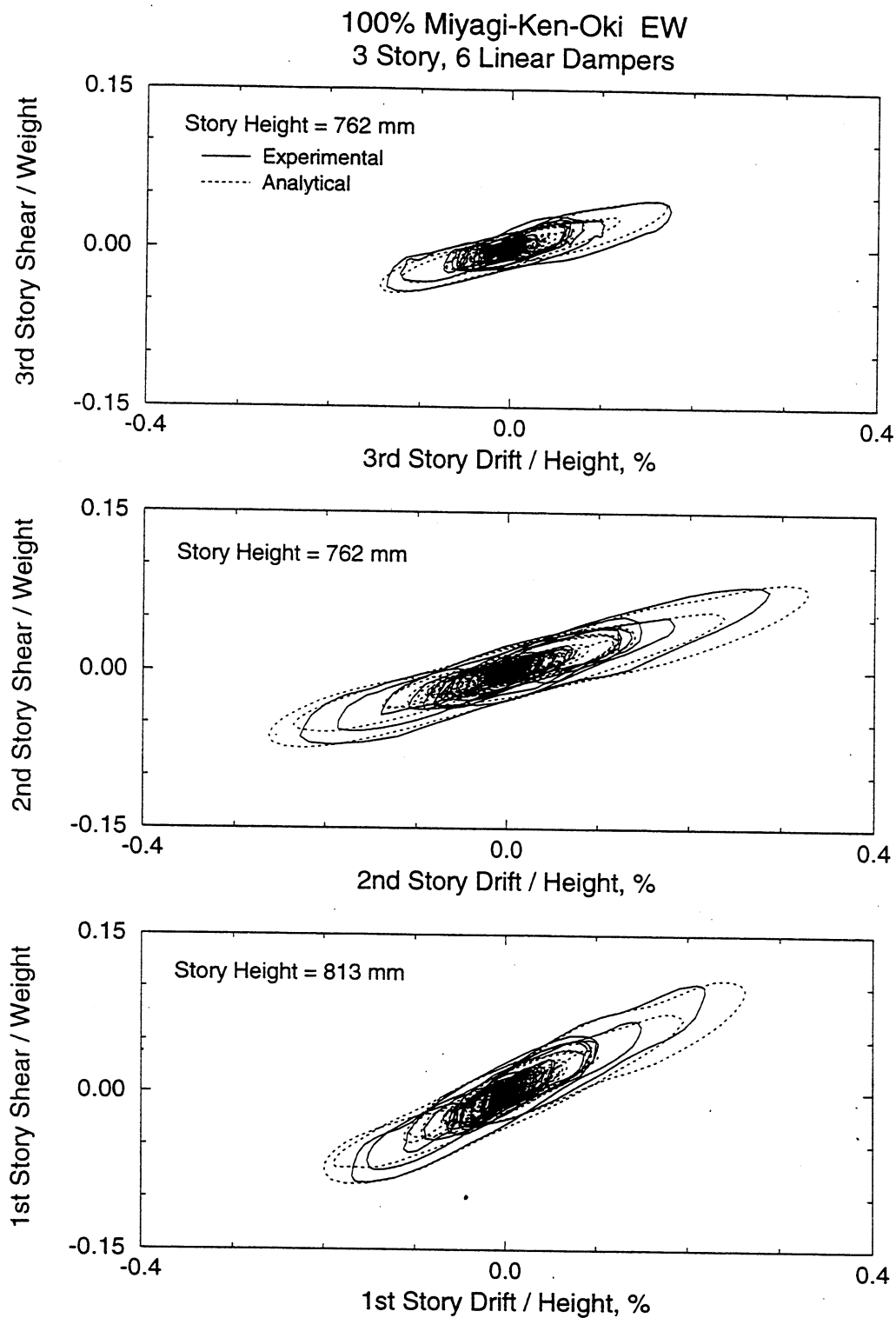
FIGURE 6-12 Comparison of Experimental and Analytical Results of 3-Story Repaired Structure with Six Linear Dampers Subjected to 100% Miyagi-Ken-Okī Earthquake
