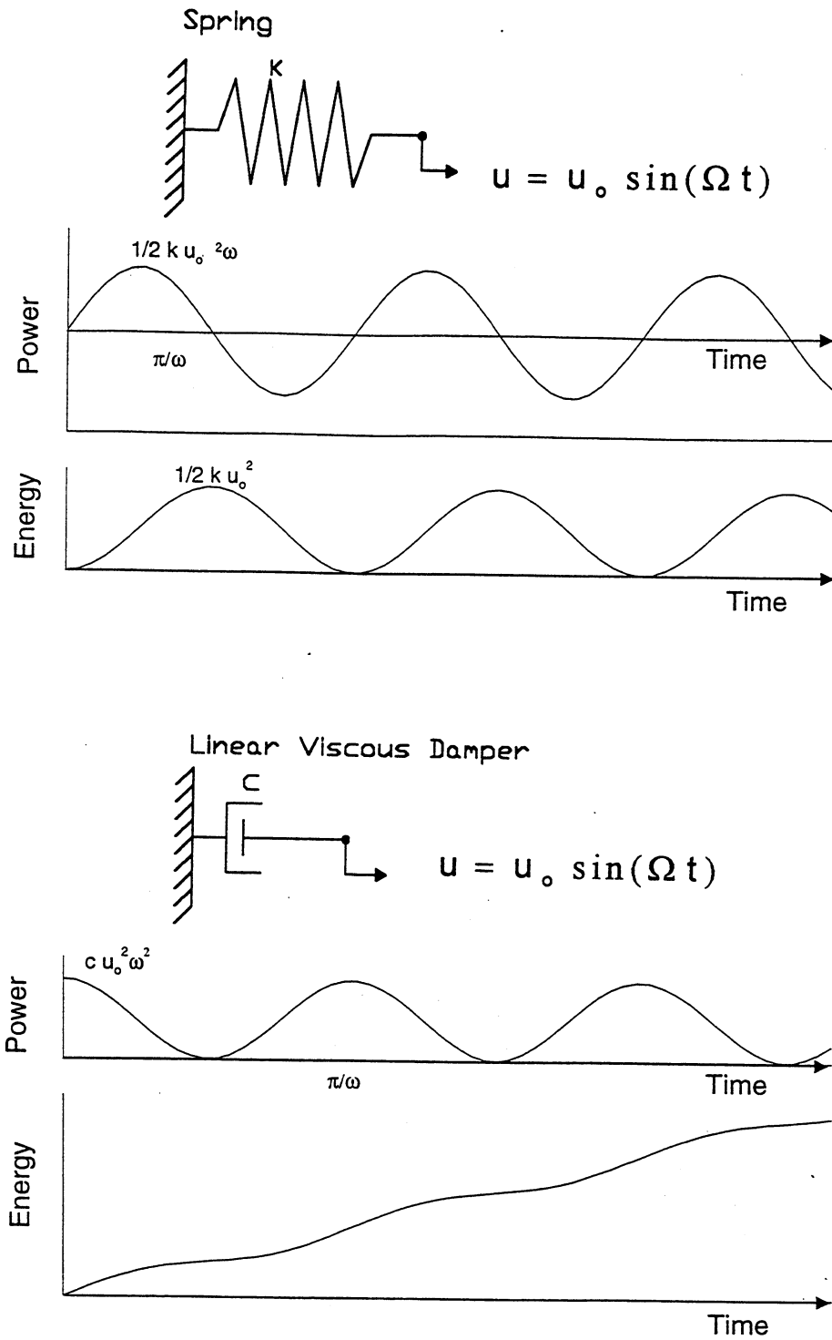
FIGURE 5-48 Comparison of Power, and Energy Time Histories of a Spring and a Linear Viscous Damper Subjected to Sinusoidal Motion
