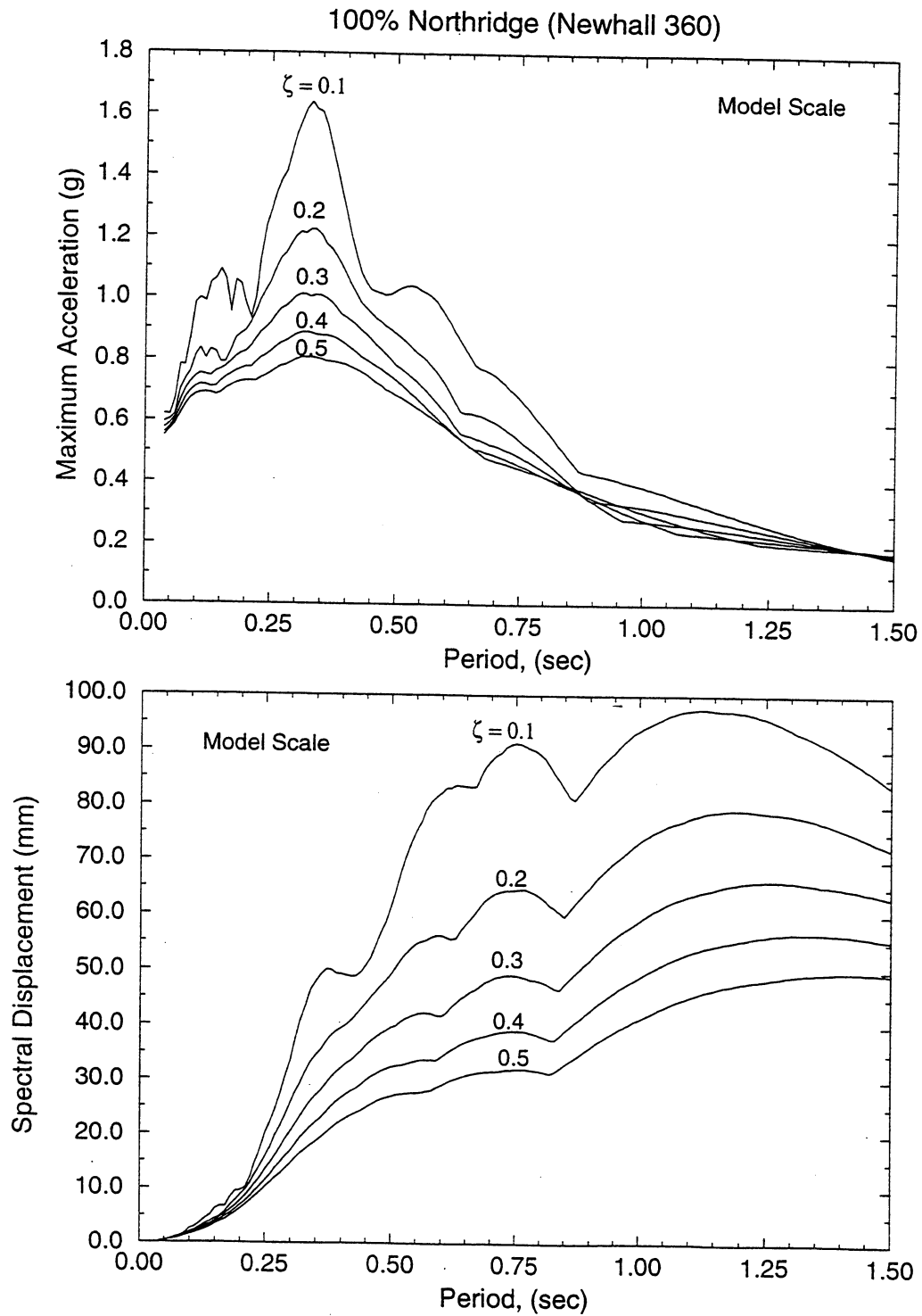
FIGURE 3-19 Time Histories of Displacement, Velocity, and Acceleration and Spectra of Acceleration and Displacement of Shaking Table Motion in 100% Northridge (Newhall 360) (Continued)
