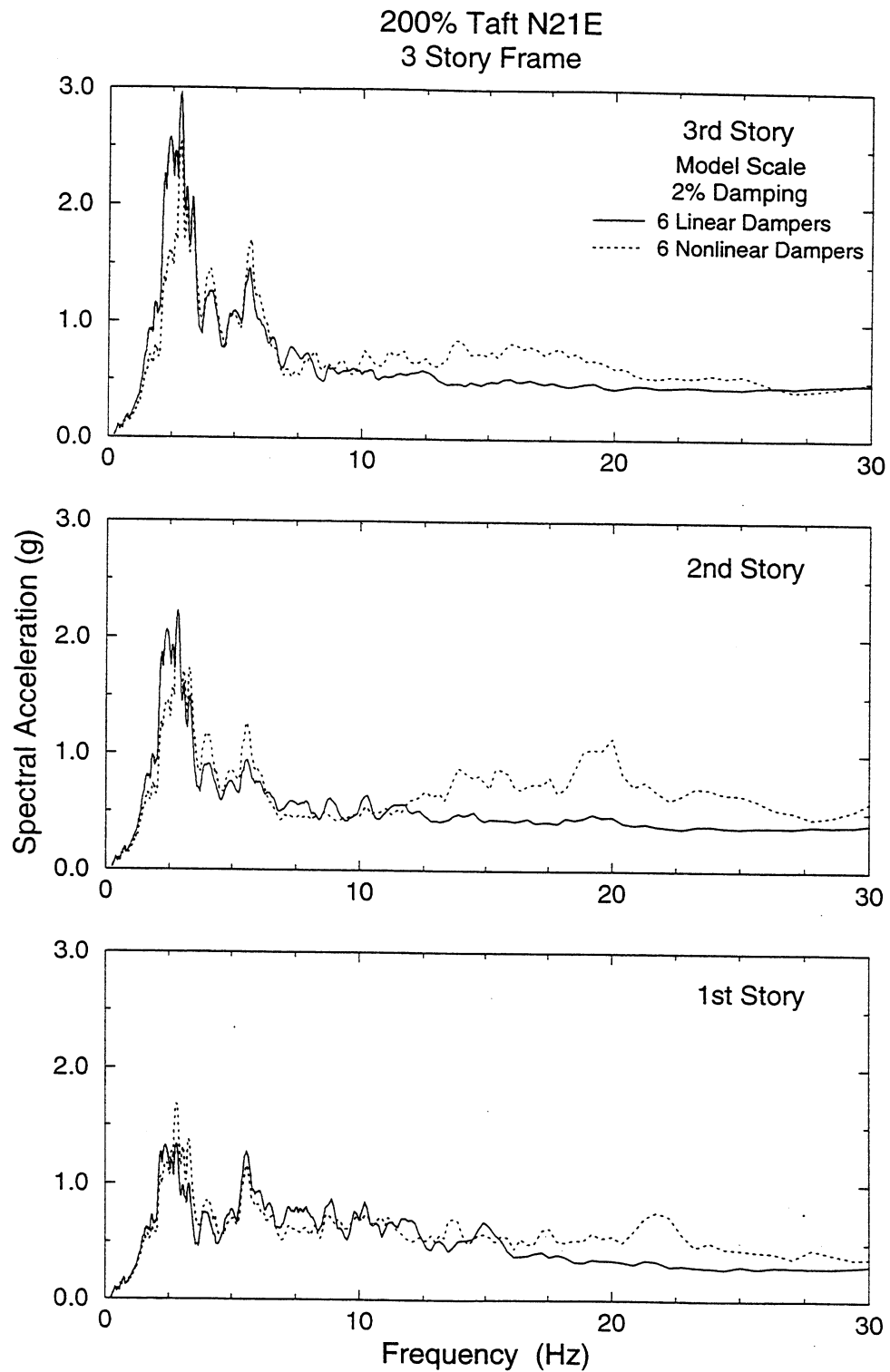
FIGURE 5-38 Comparison of Floor Response Spectra of 3-Story Repaired Structure with Six Linear and Six Nonlinear Dampers Subjected to 200% Taft Earthquake
