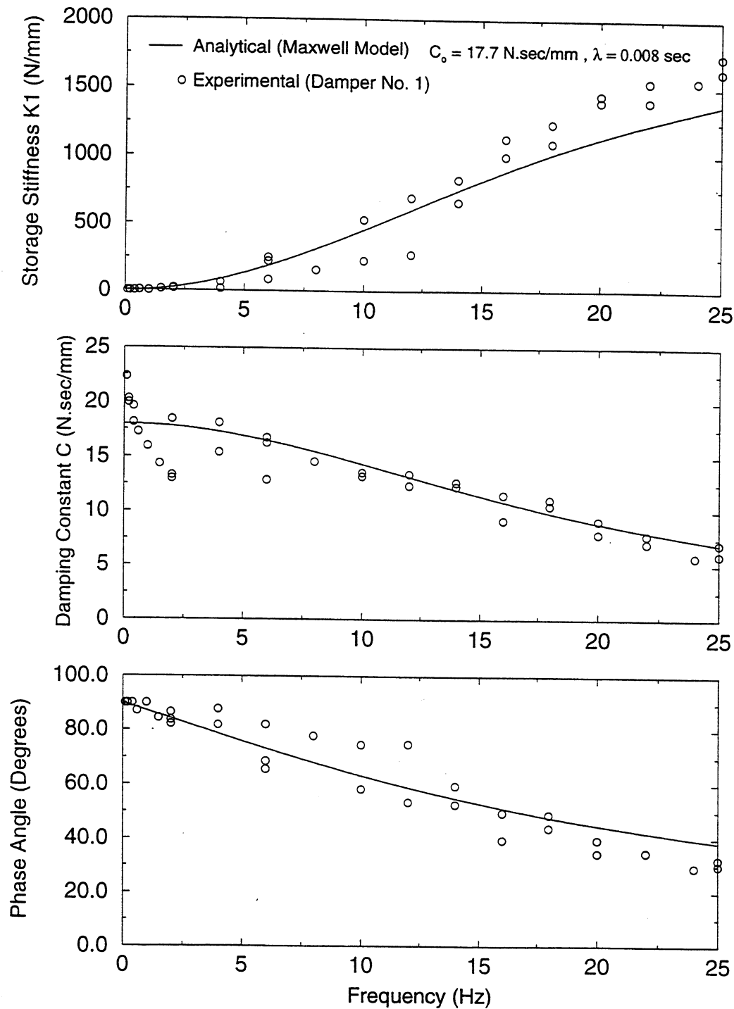
FIGURE 2-11 Comparison of Experimental and Analytically Derived Values of Storage Stiffness, Damping Constant and Phase Angle for Linear Dampers
