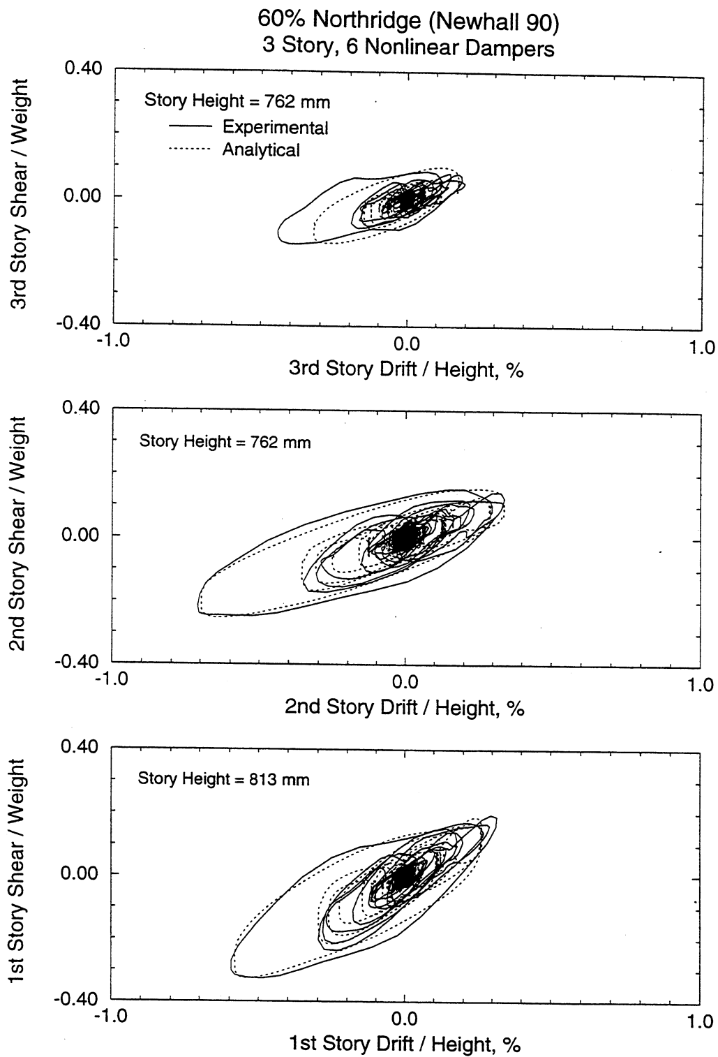
FIGURE 6-21 Comparison of Experimental and Analytical Results of 3-Story Repaired Structure with Six Nonlinear Dampers Subjected to 60% Northridge (Newhall 90) Earthquake
