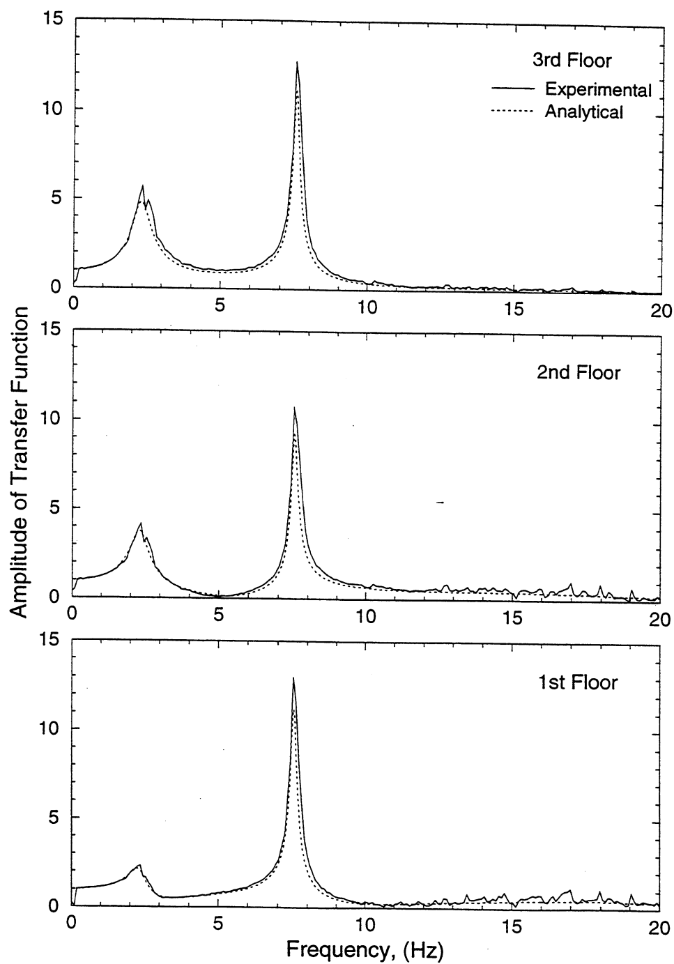
FIGURE 4-6 Comparison of Analytical and Experimental Transfer Functions of 3-Story Repaired Frame with Two Linear Dampers at Second Story
