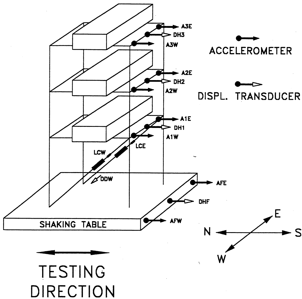
FIGURE 3-23 Instrumentation Diagram
