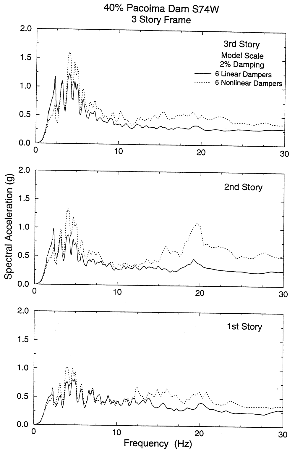
FIGURE 5-42 Comparison of Floor Response Spectra of 3-Story Repaired Structure with Six Linear and Six Nonlinear Dampers Subjected to 40% Pacoima Dam Earthquake
