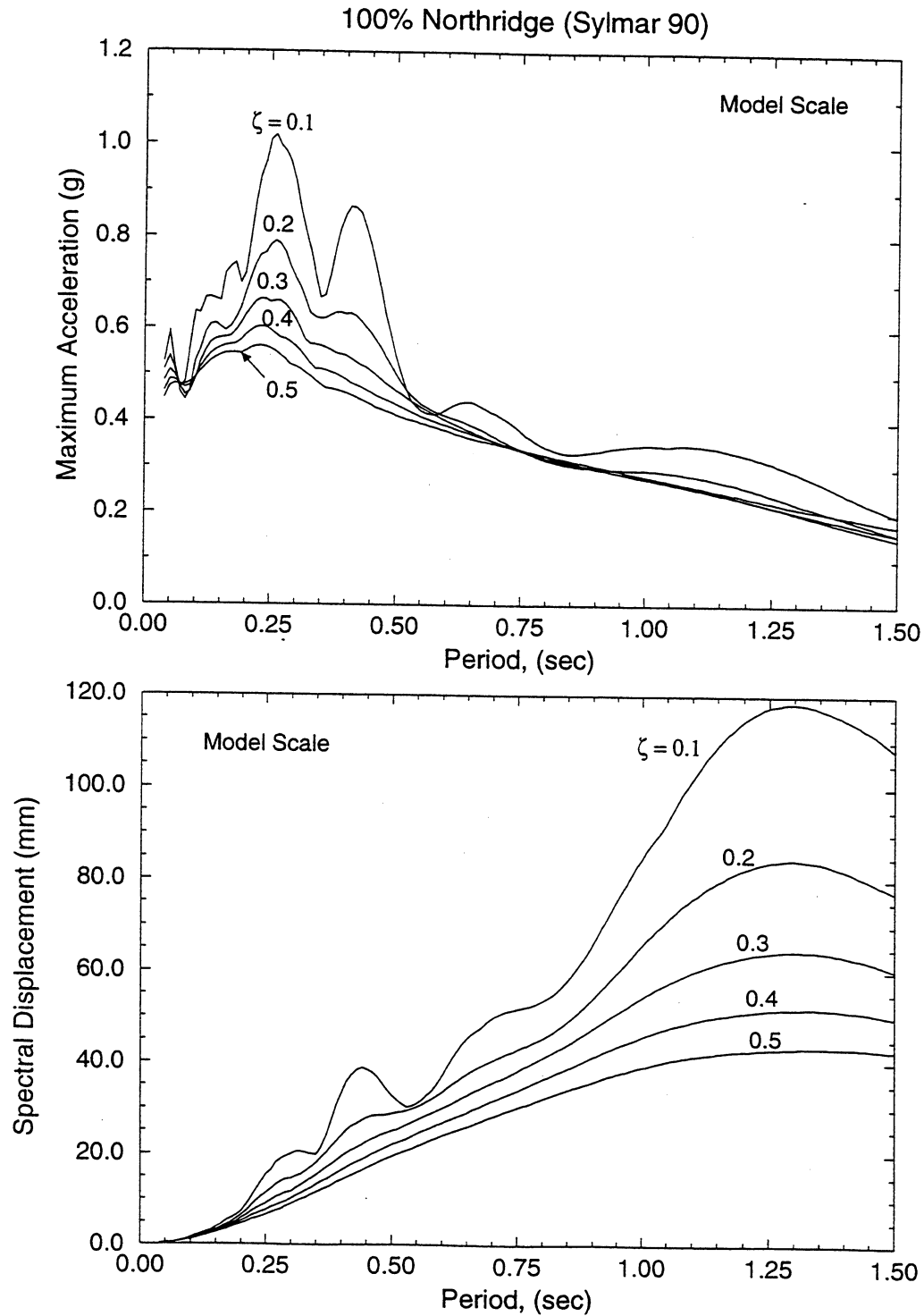
FIGURE 3-20 Time Histories of Displacement, Velocity, and Acceleration and Spectra of Acceleration and Displacement of Shaking Table Motion in 100% Northridge (Sylmar 90) (Continued)
