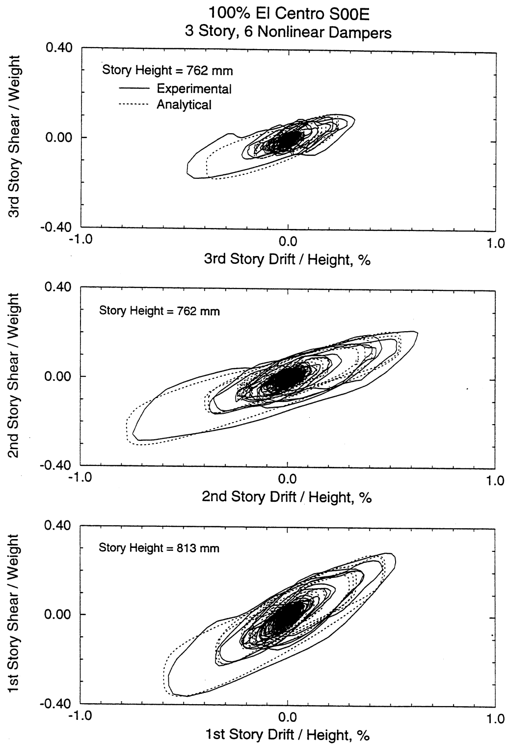
FIGURE 6-19 Comparison of Experimental and Analytical Results of 3-Story Repaired Structure with Six Nonlinear Dampers Subjected to 100% El Centro Earthquake
