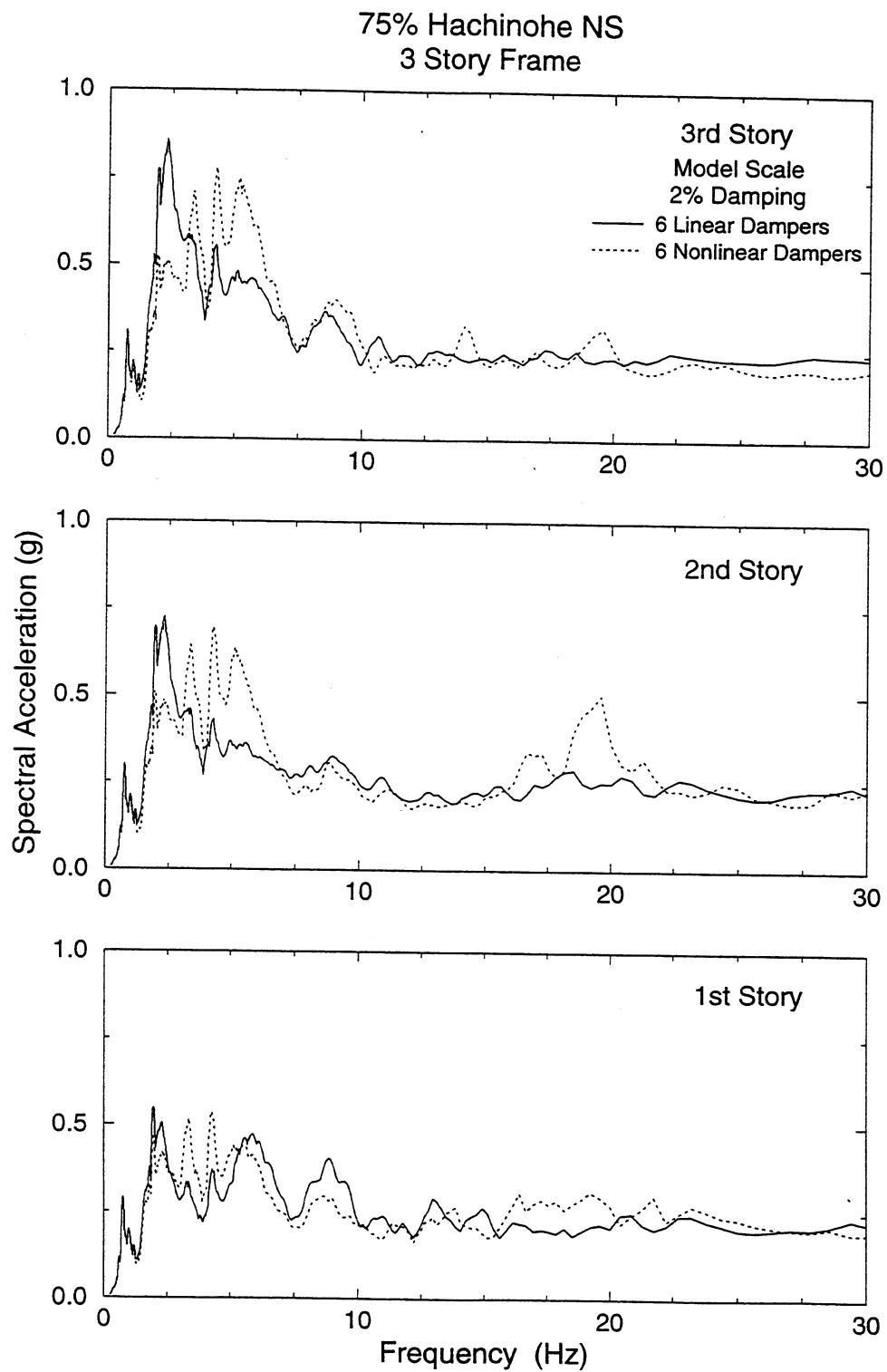
FIGURE 5-43 Comparison of Floor Response Spectra of 3-Story Repaired Structure with Six Linear and Six Nonlinear Dampers Subjected to 75% Hachinohe Earthquake
