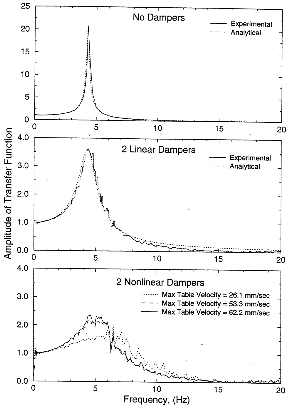
FIGURE 4-1 Transfer Functions of One-Story Frame without and with Two Linear and Two Nonlinear Dampers
