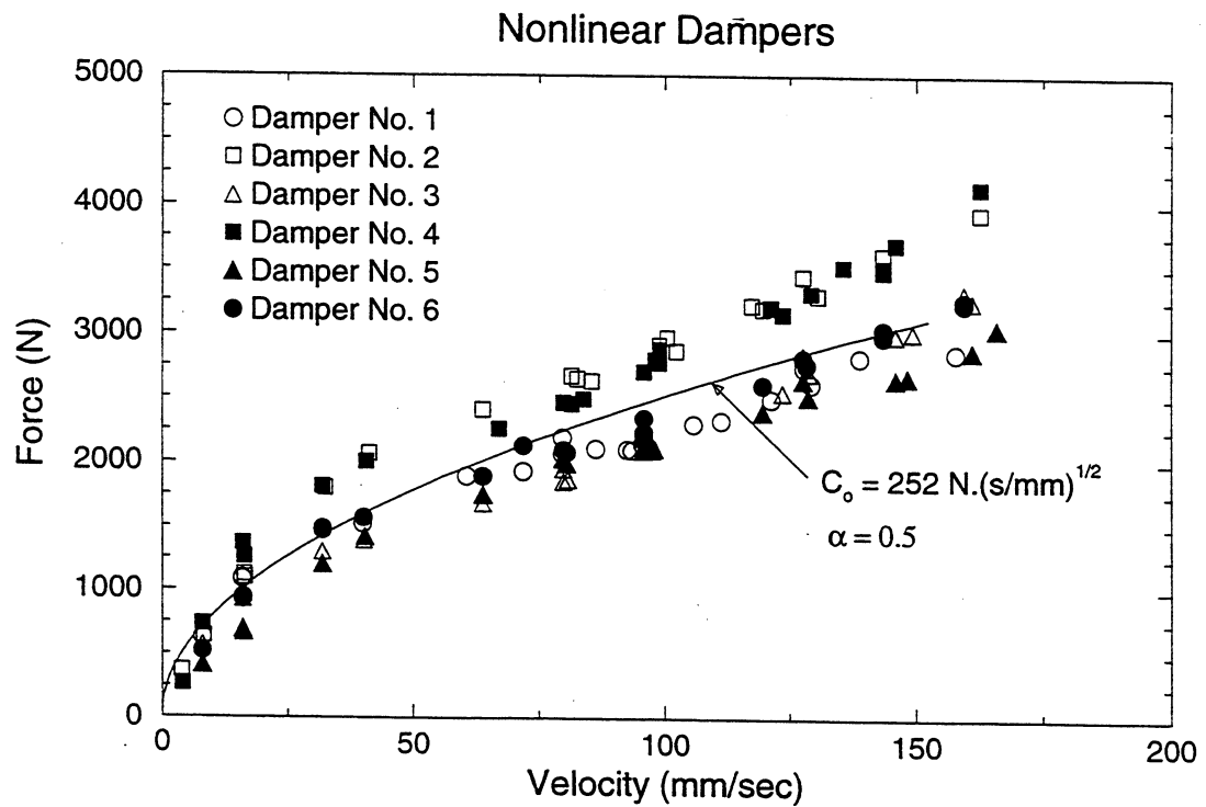
FIGURE 2-8 Force-Velocity Relationship of Linear and Nonlinear Dampers
