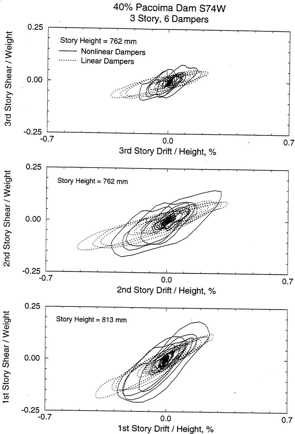
FIGURE 5-31 Comparison of Normalized Shear-Drift Loops of 3-Story Repaired Structure with Six Linear and Six Nonlinear Dampers Subjected to 40% Pacoima Dam Earthquake
