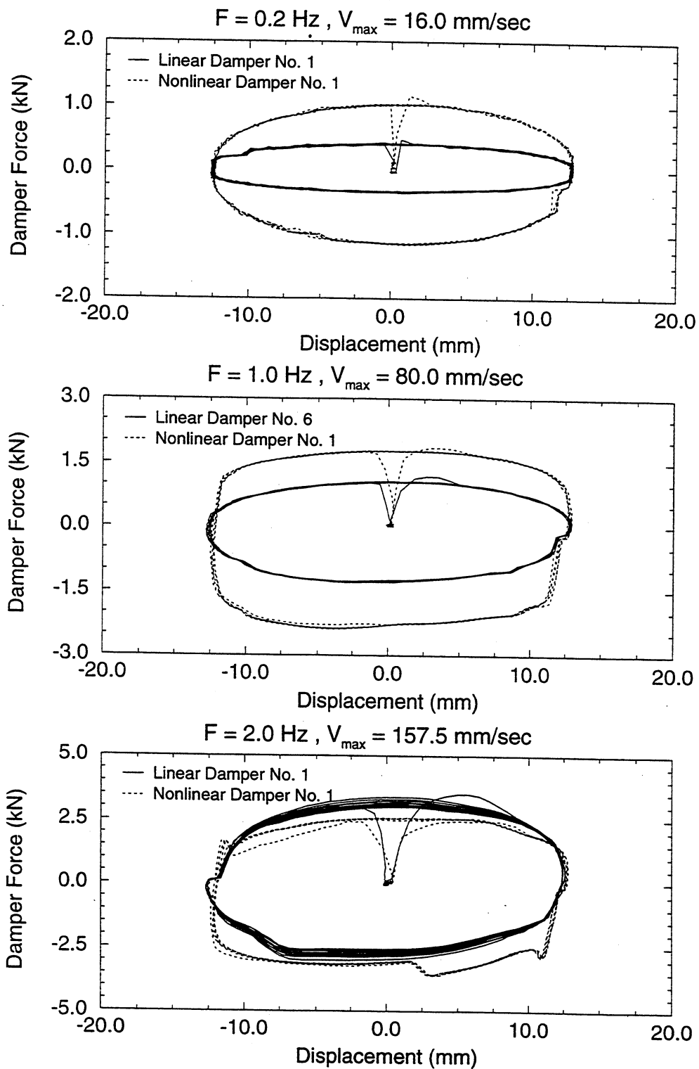
FIGURE 2-7 Comparison between Linear and Nonlinear Damper Loops
