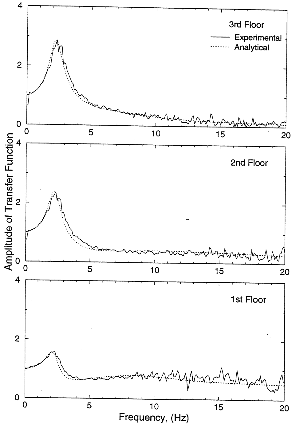
FIGURE 4-8 Comparison of Analytical and Experimental Transfer Functions of 3-Story Repaired Frame with Six Linear Dampers at All Stories (Two at Each Story)
