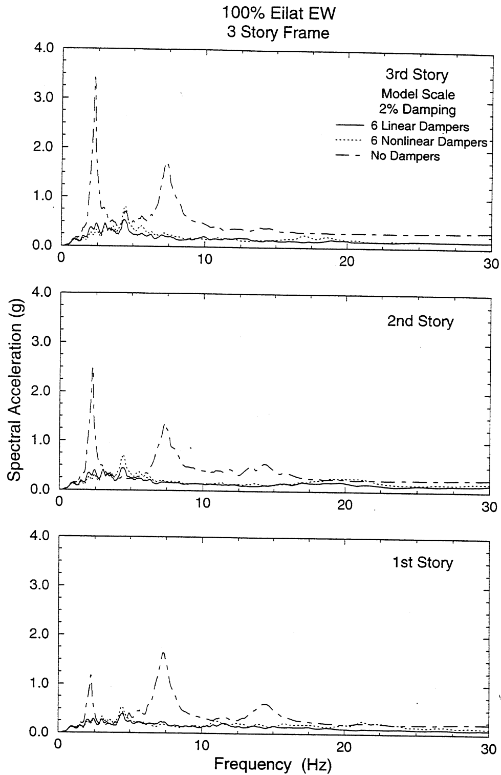
FIGURE 5-35 Comparison of Floor Response Spectra of 3-Story Repaired Structure without, with Six Linear and with Six Nonlinear Dampers Subjected to 100% Eilat EW Earthquake
