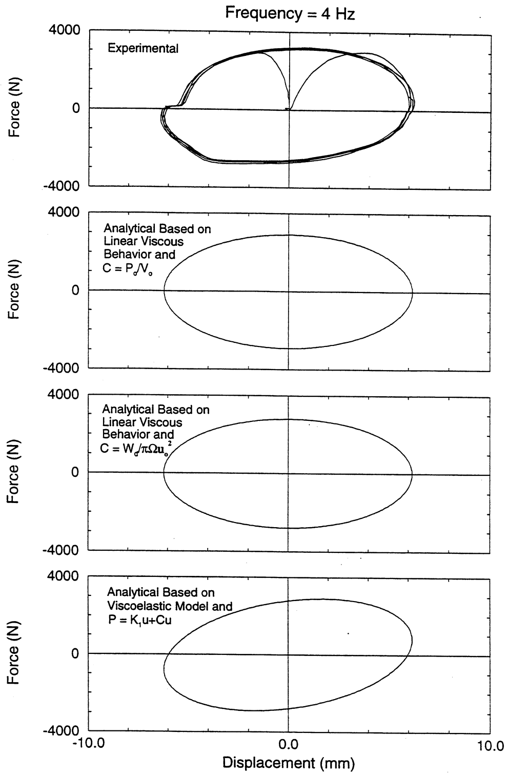
FIGURE 2-4 Example of Model Calibration
