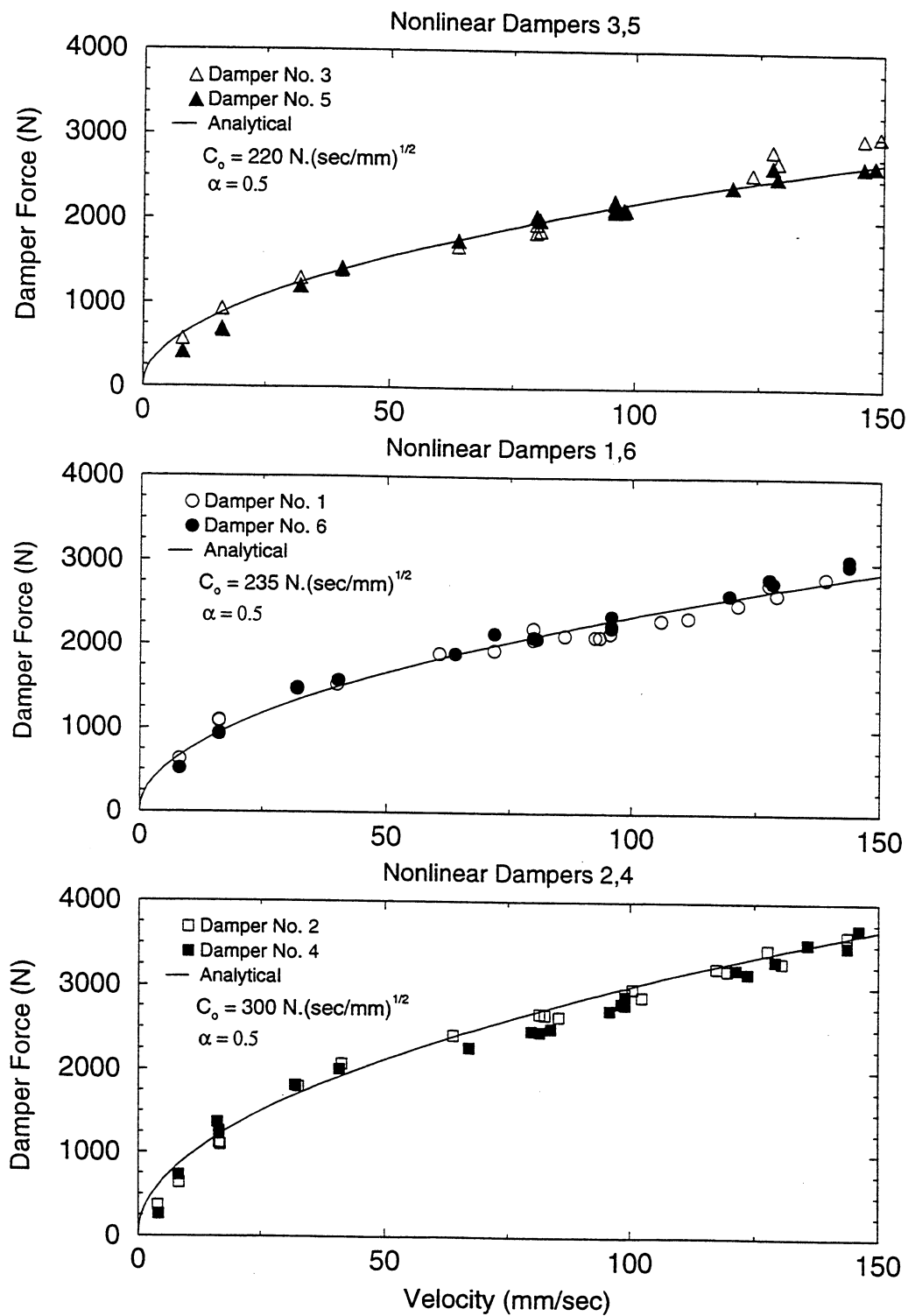
FIGURE 2-10 Refined Model for Nonlinear Dampers
