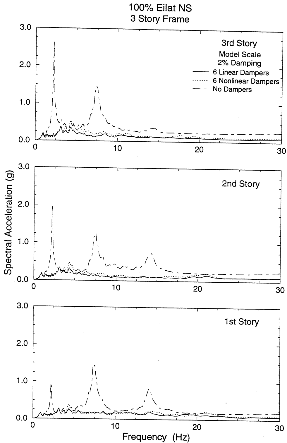
FIGURE 5-34 Comparison of Floor Response Spectra of 3-Story Repaired Structure without, with Six Linear and with Six Nonlinear Dampers Subjected to 100% Eilat NS Earthquake
