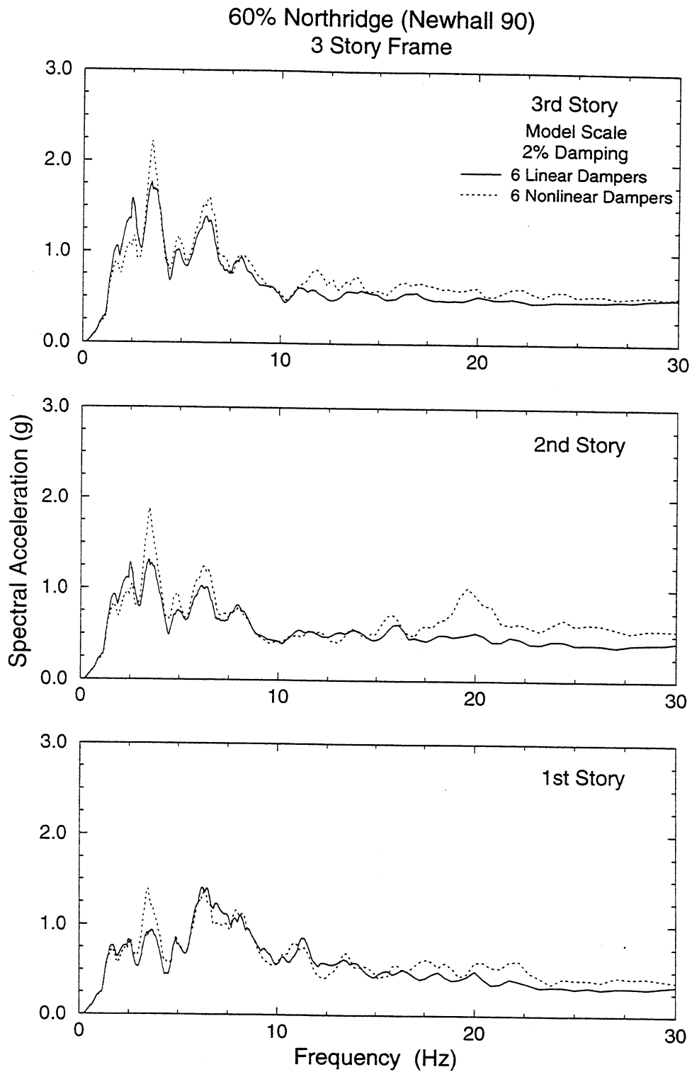
FIGURE 5-39 Comparison of Floor Response Spectra of 3-Story Repaired Structure with Six Linear and Six Nonlinear Dampers Subjected to 60% Northridge (Newhall 90) Earthquake
