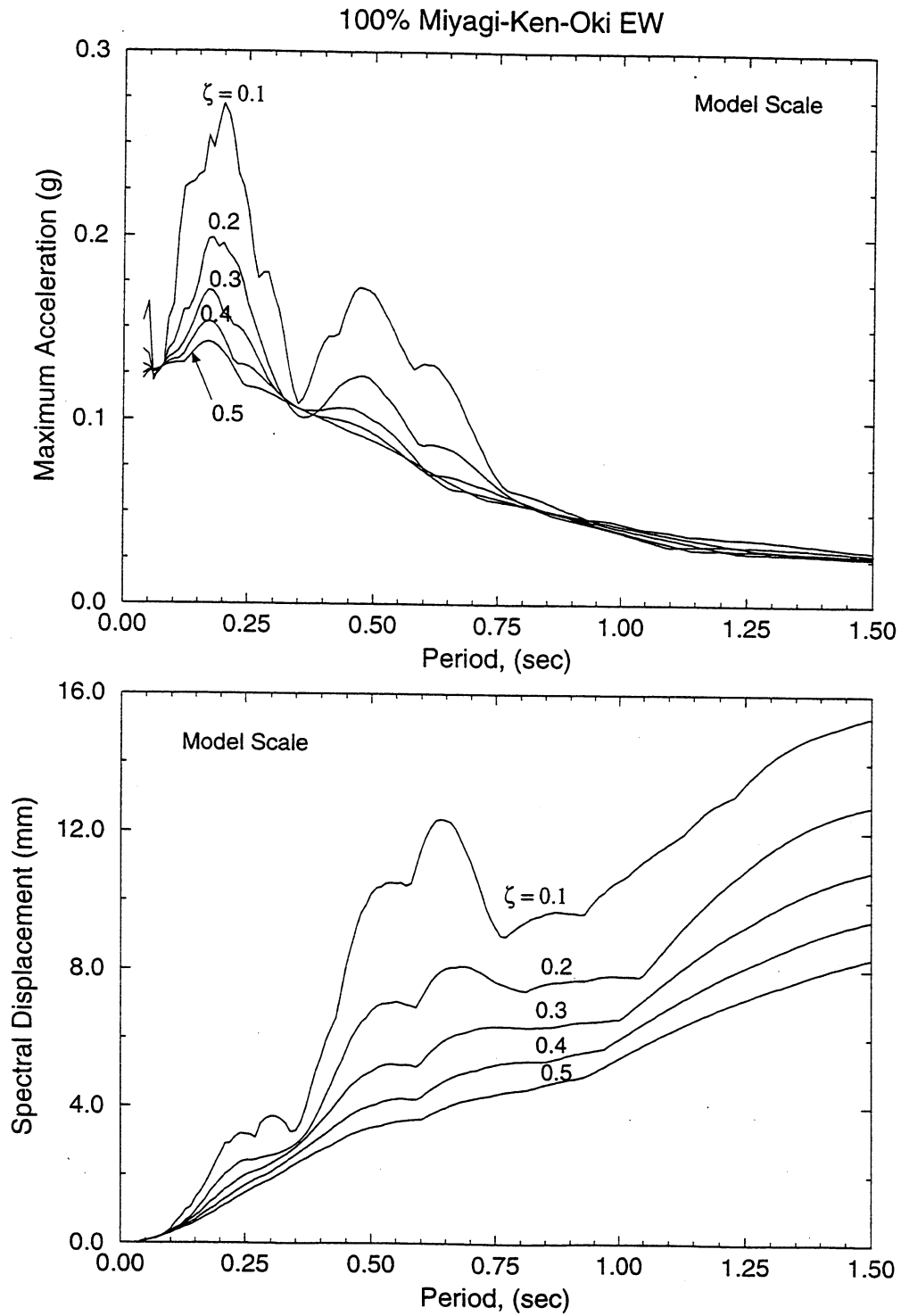
FIGURE 3-16 Time Histories of Displacement, Velocity, and Acceleration and Spectra of Acceleration and Displacement of Shaking Table Motion in 100% Miyagi-Ken-Oki EW (Continued)
