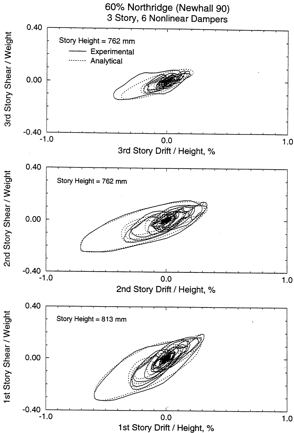
FIGURE 6-27 Comparison of Experimental and Analytical Results of 3-Story Repaired Structure with Six Nonlinear Dampers Subjected to 60% Northridge (Newhall 90) Earthquake (Refined Model of Nonlinear Dampers)
