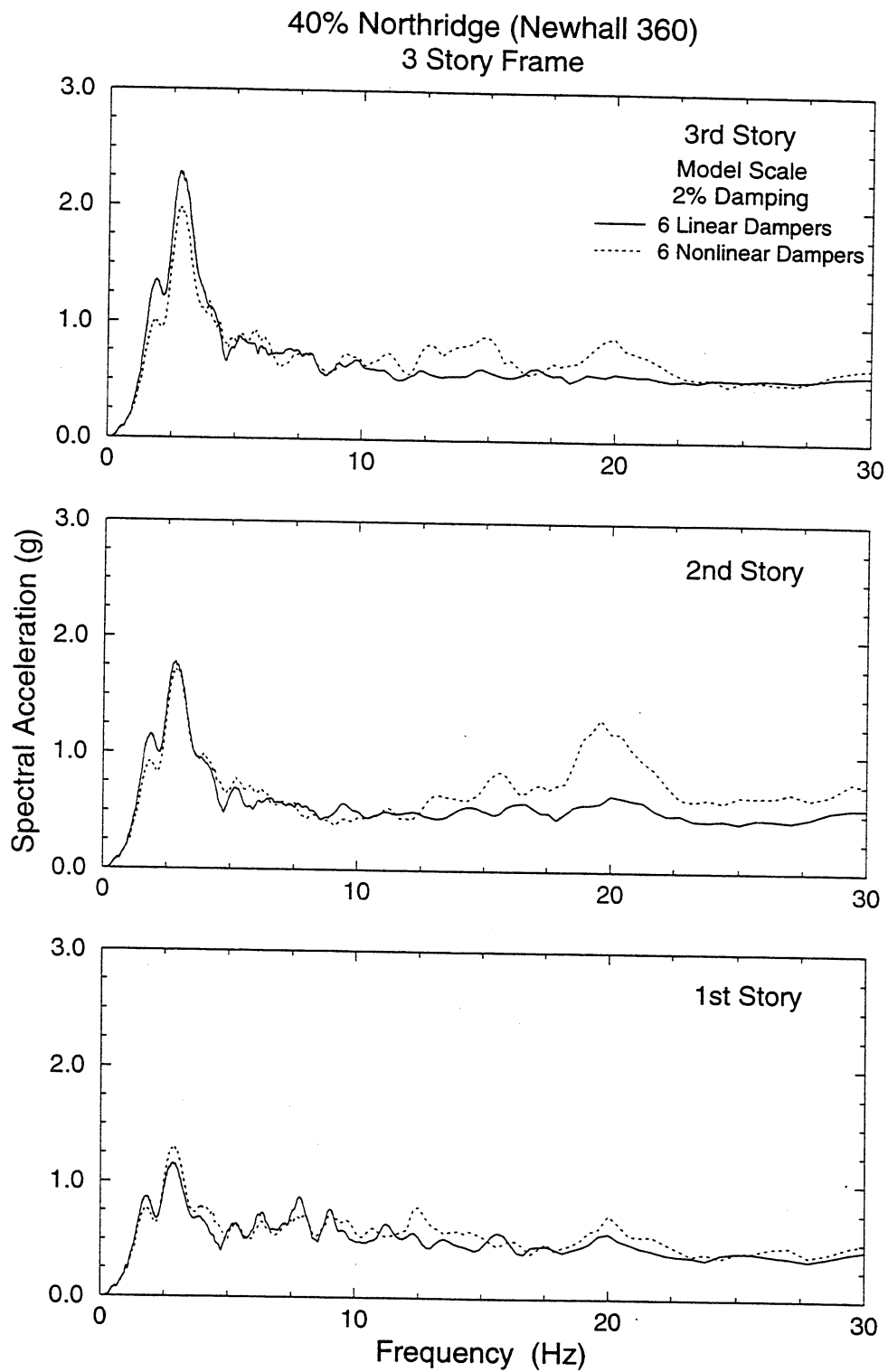
FIGURE 5-40 Comparison of Floor Response Spectra of 3-Story Repaired Structure with Six Linear and Six Nonlinear Dampers Subjected to 40% Northridge (Newhall 360) Earthquake
