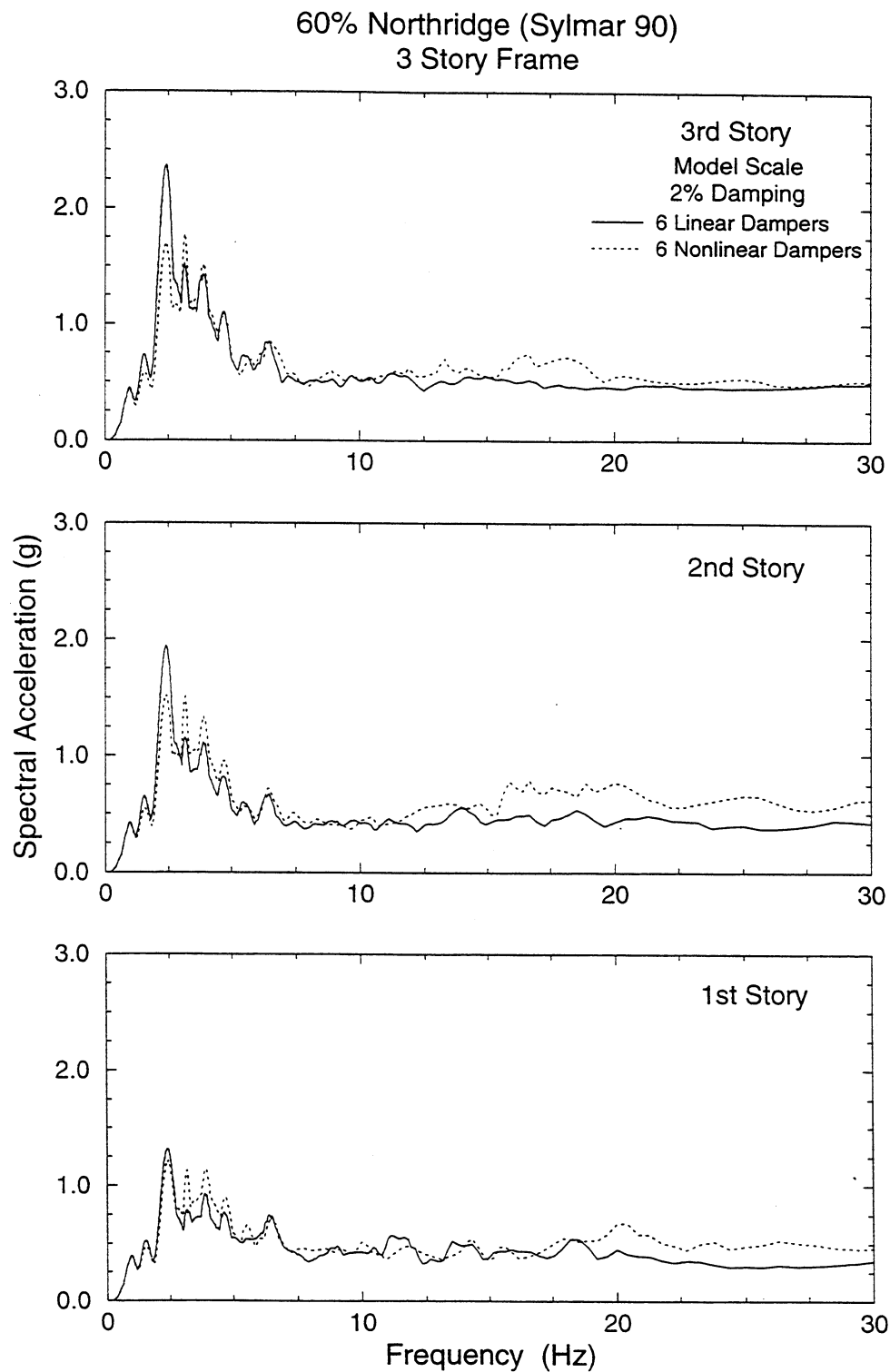
FIGURE 5-41 Comparison of Floor Response Spectra of 3-Story Repaired Structure with Six Linear and Six Nonlinear Dampers Subjected to 60% Northridge (Sylmar 90) Earthquake
