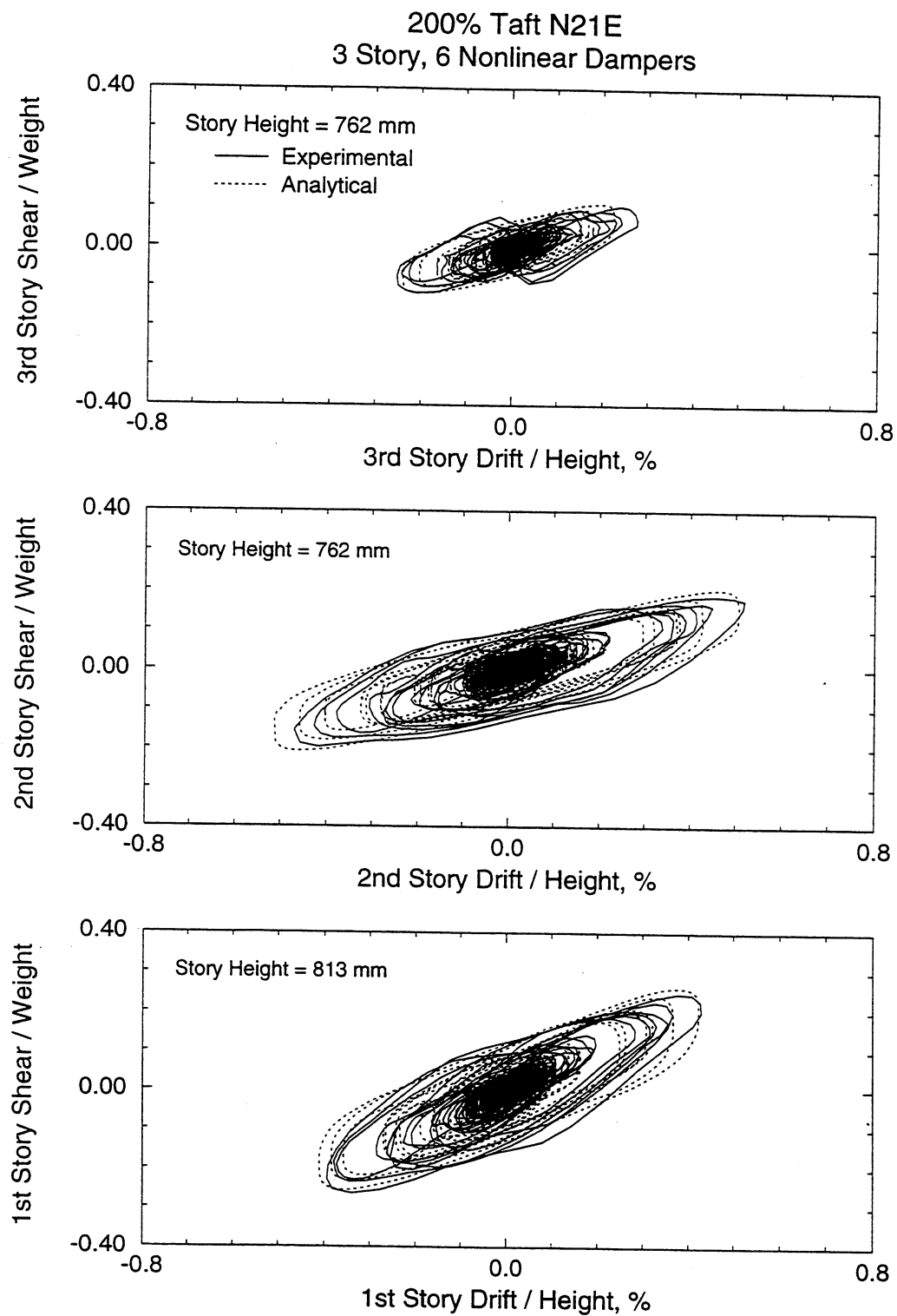
FIGURE 6-20 Comparison of Experimental and Analytical Results of 3-Story Repaired Structure with Six Nonlinear Dampers Subjected to 200% Taft Earthquake
