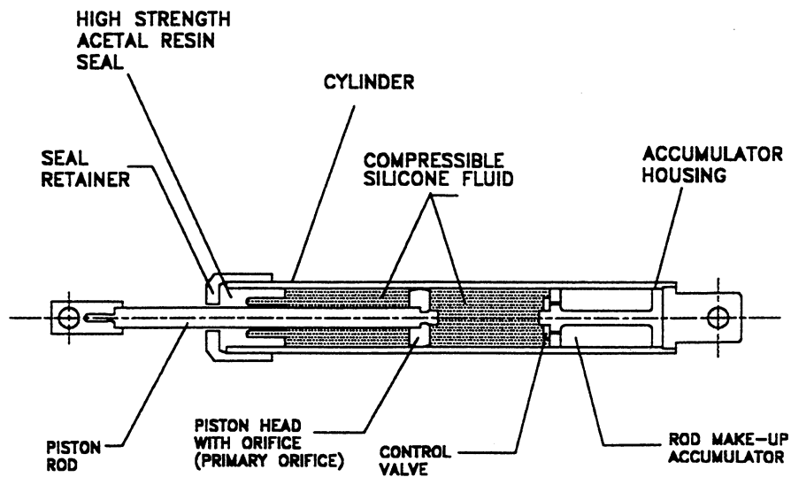
FIGURE 2-1 Longitudinal Cross Section of a Fluid Damper
