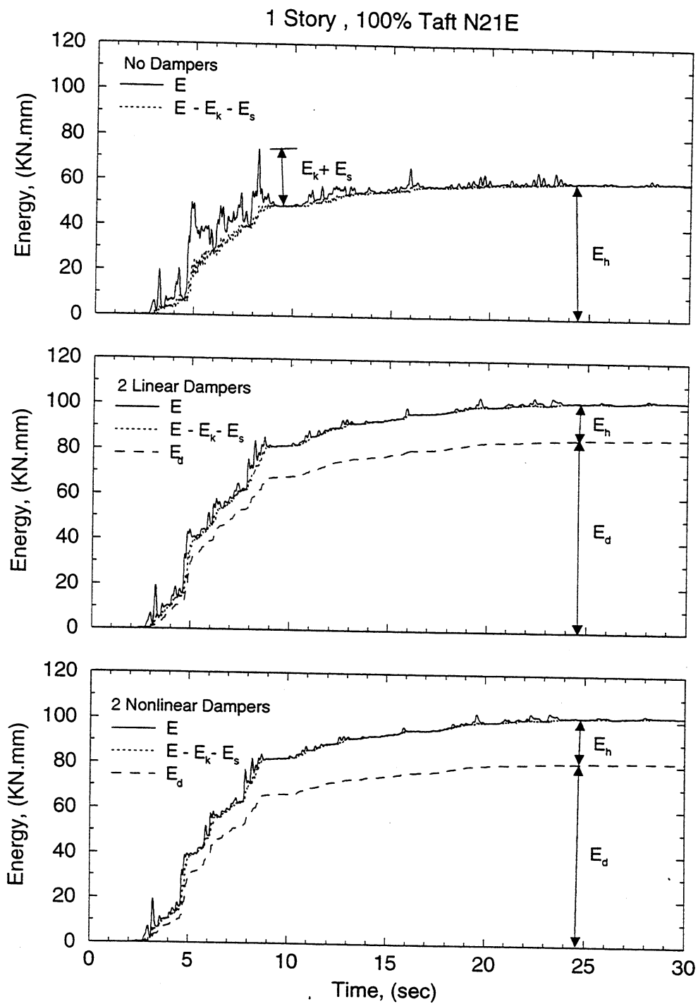
FIGURE 5-45 Energy Time Histories of One-Story Structure without, with Two Linear and with Two Nonlinear Dampers Subjected to 100% Taft Earthquake
