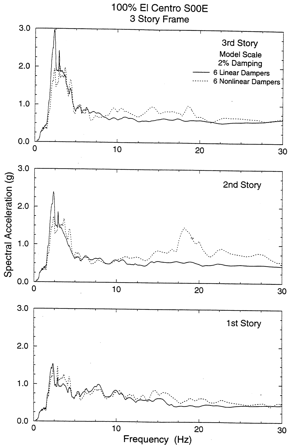
FIGURE 5-37 Comparison of Floor Response Spectra of 3-Story Repaired Structure with Six Linear and Six Nonlinear Dampers Subjected to 100% El Centro Earthquake
