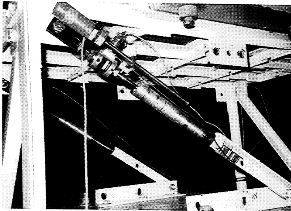
FIGURE 3-11 Close-up View of the Dampers
