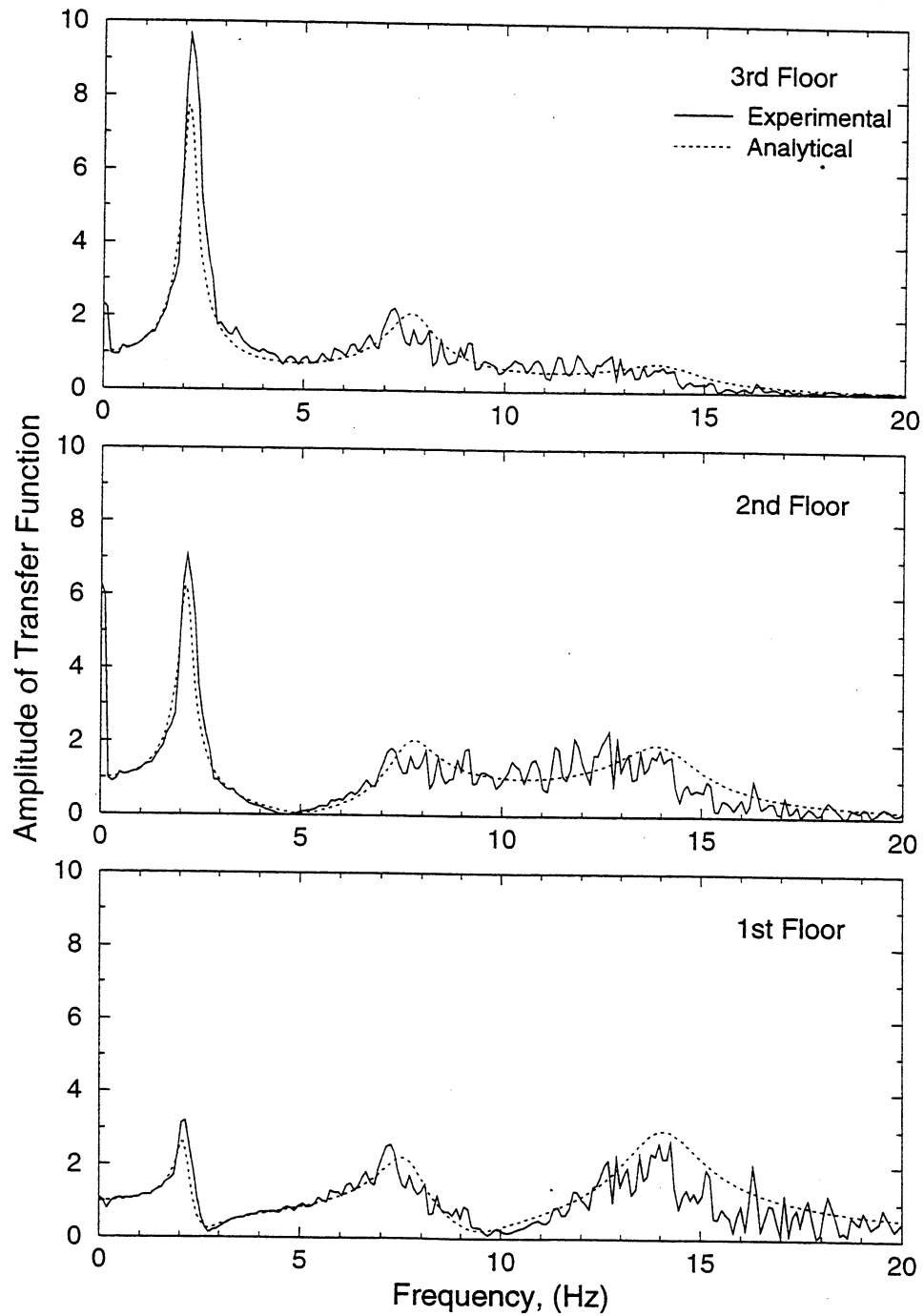
FIGURE 4-5 Comparison of Analytical and Experimental Transfer Functions of 3-Story Frame (Prior to Repair with 16 Tapered Plates) with Two Linear Dampers at First Story.
