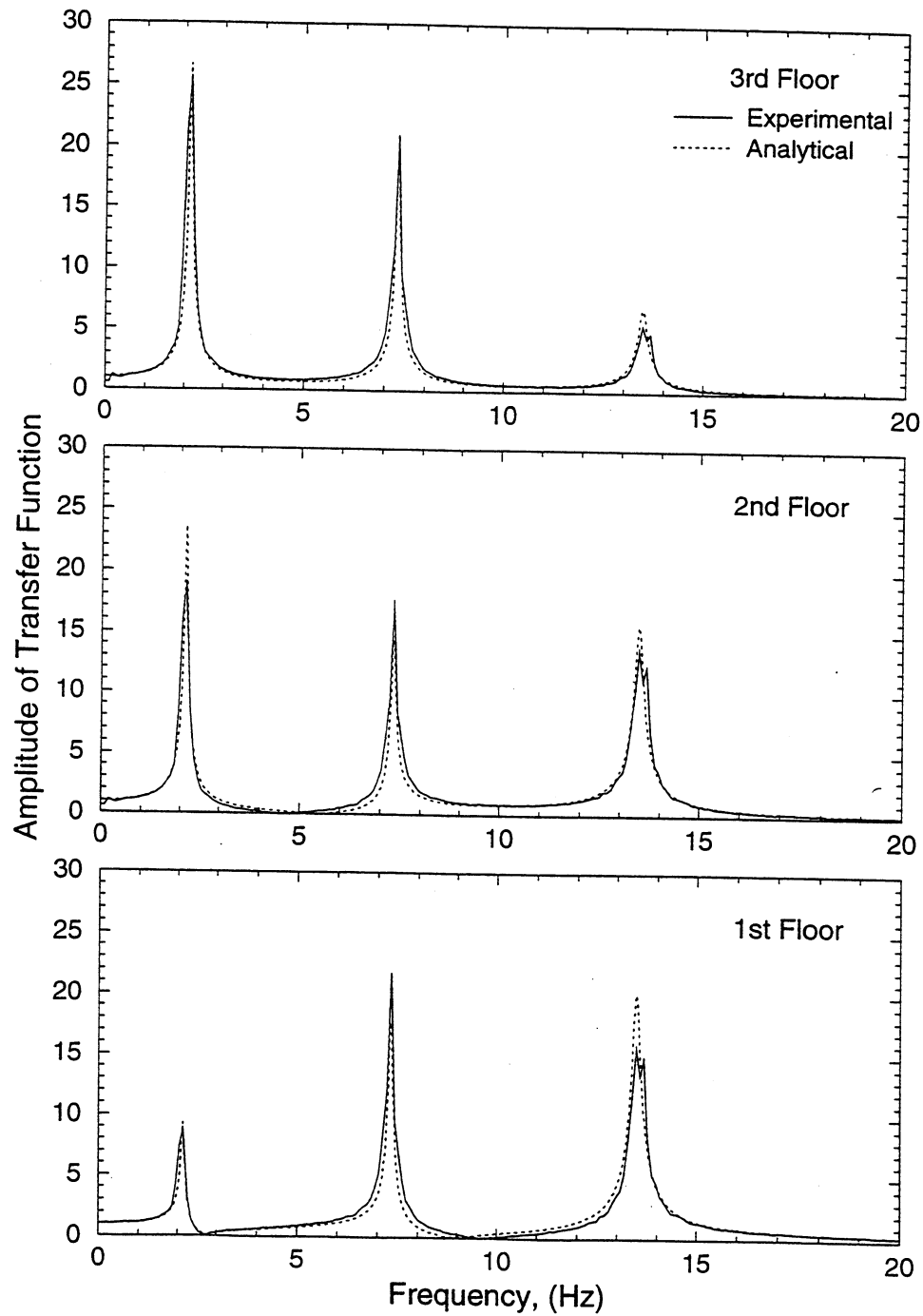
FIGURE 4-3 Comparison of Analytical and Experimental Transfer Functions of 3-Story Cracked Frame without Dampers (Prior to Repair with 16 Tapered Plates)
