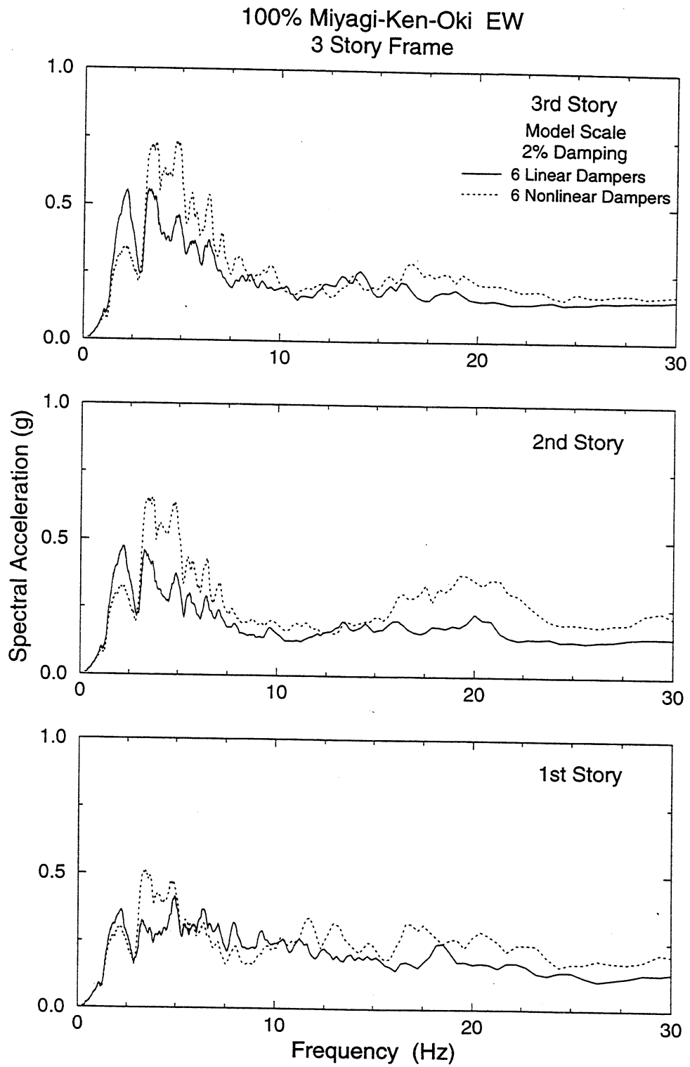
FIGURE 5-44 Comparison of Floor Response Spectra of 3-Story Repaired Structure with Six Linear and Six Nonlinear Dampers Subjected to 100% Miyagi-Ken-Oki Earthquake
