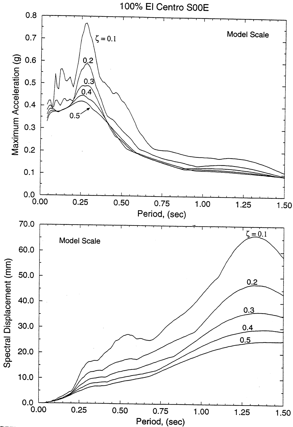
FIGURE 3-13 Time Histories of Displacement, Velocity, and Acceleration, and Spectra of Acceleration and Displacement of Shaking Table Motion in 100% El Centro S00E (Continued)
