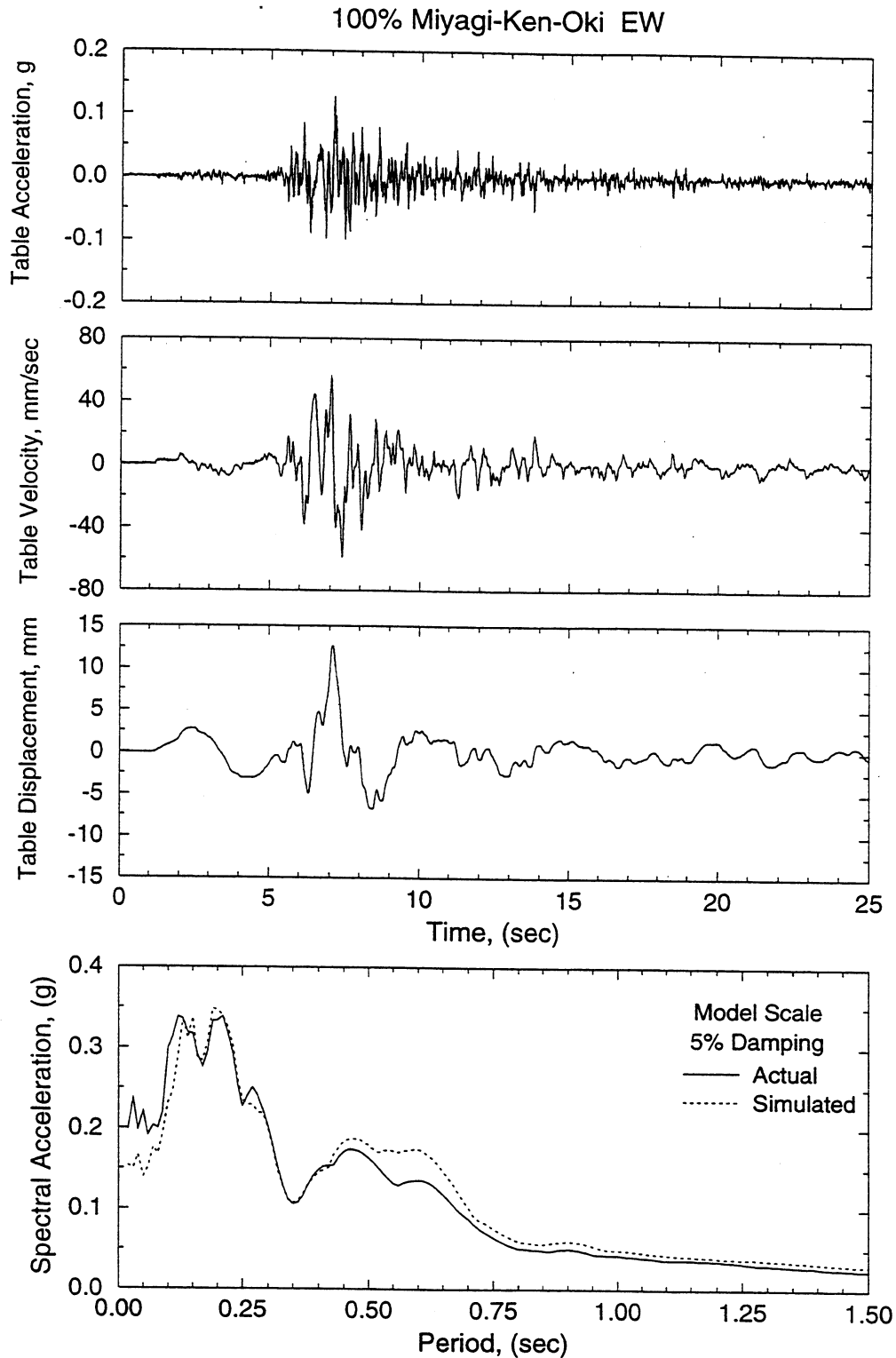
FIGURE 3-16 Time Histories of Displacement, Velocity, and Acceleration and Spectra of Acceleration and Displacement of Shaking Table Motion in 100%Miyagi-Ken-Okai EW
