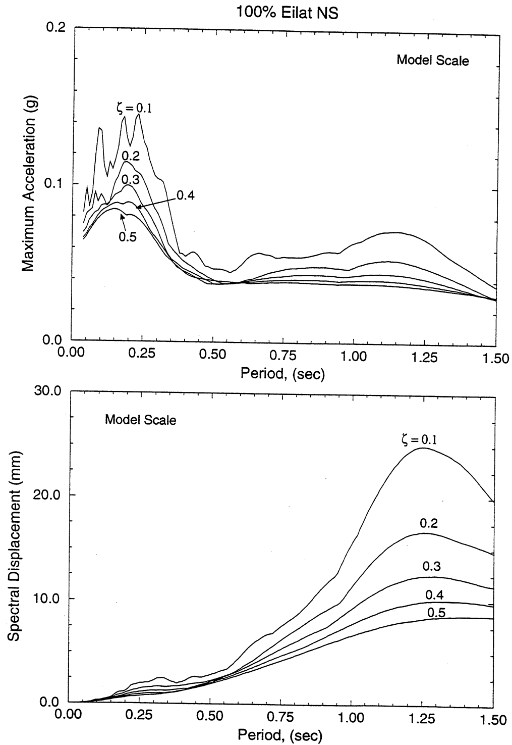
FIGURE 3-21 Time Histories of Displacement, Velocity, and Acceleration and Spectra of Acceleration and Displacement of Shaking Table Motion in 100% Eilat NS (Continued)
