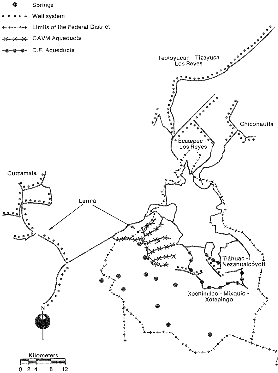
FIGURE 3-1 Water Supply For Metropolitan Mexico City
