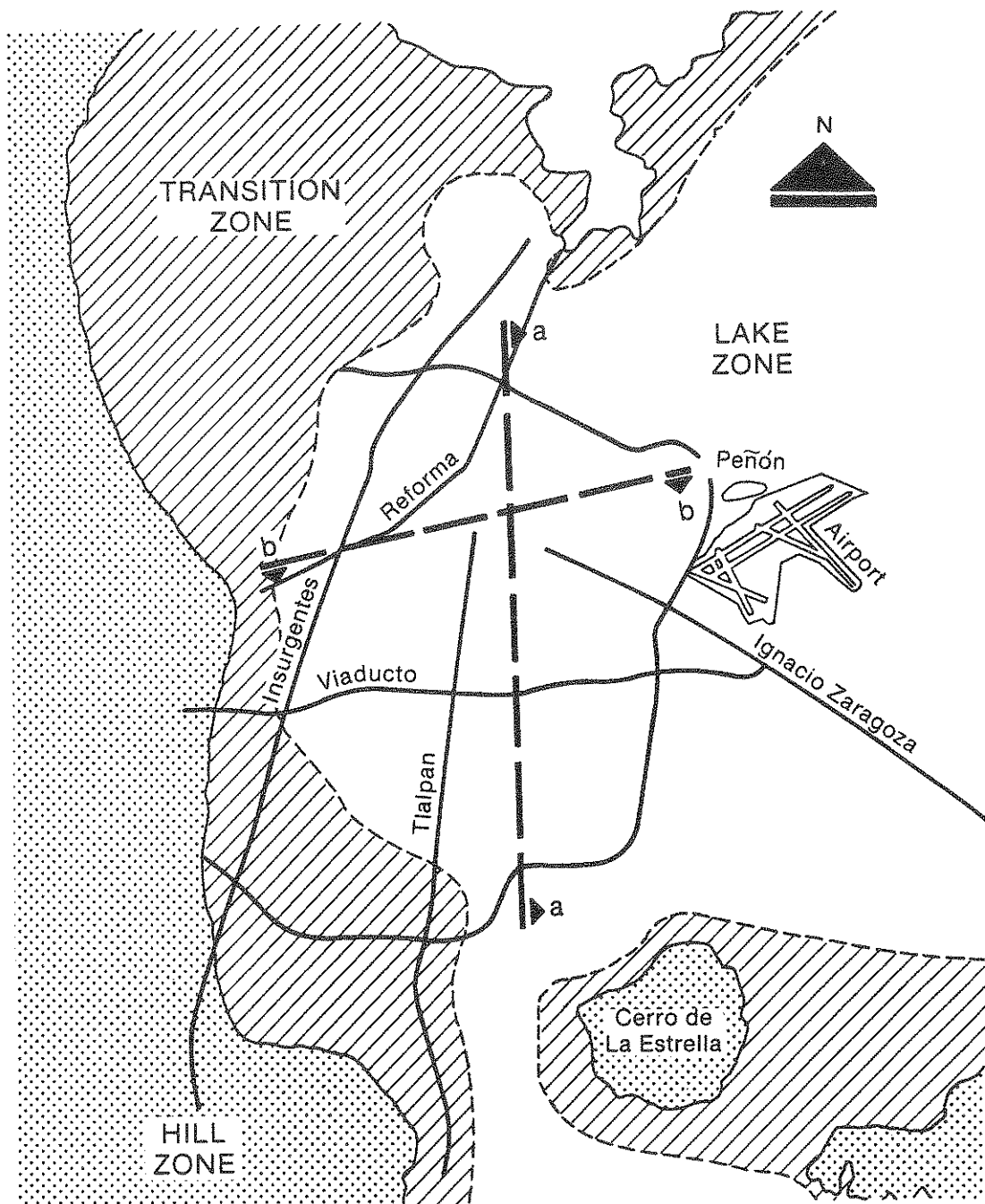
FIGURE 5-1 Soil Zones For Metropolitan Mexico City
