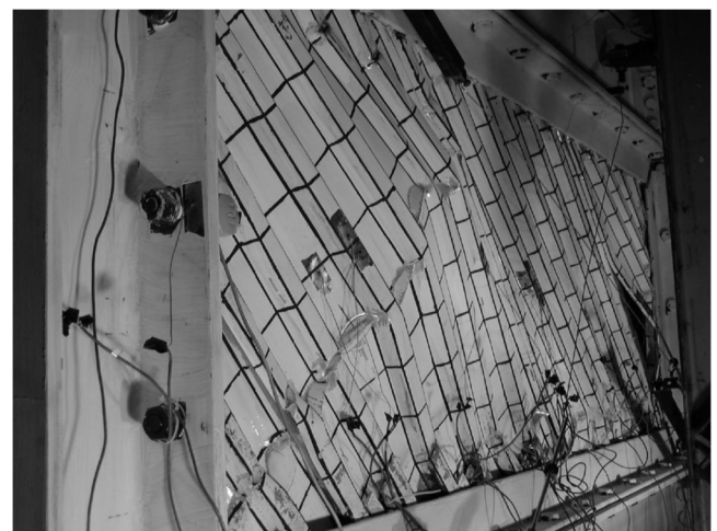
Fig. 11. Global and local buckling of Specimen C1 at -3\Delta_y of Cycle 16
