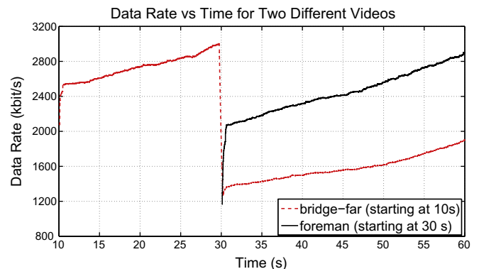
Fig. 5. The data rate of two different quality videos starting at different times.
