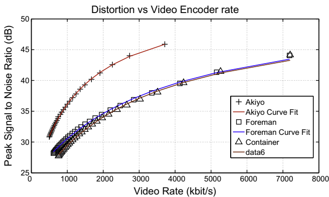
Fig. 1. Regression curves used to determine distortion due to JPEG encoding.
