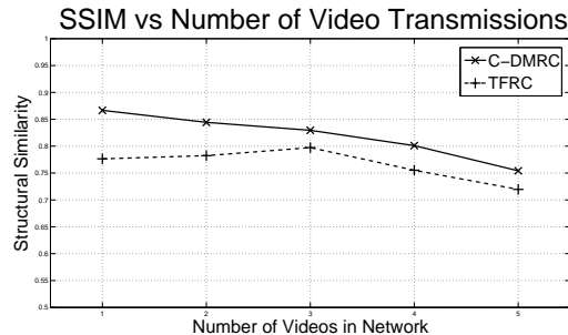
Fig. 12. SSIM of a multiple video transmissions using C-DMRC and TFRC.
