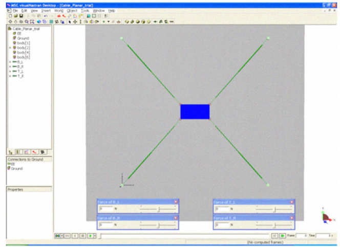
Fig. 4. The configuration of the planar cable robot with rigid-body end-effector under consideration modeled in MSC visualNastran.
