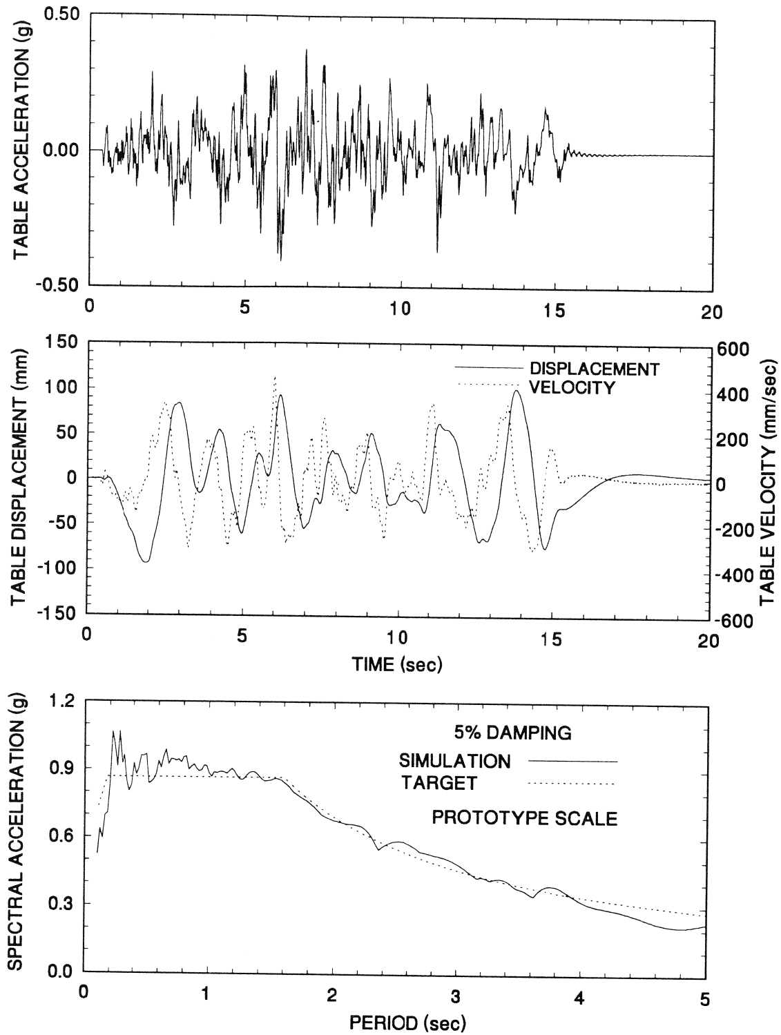
Figure 4-22 Time Histories of Displacement, Velocity and Acceleration and Acceleration Response Spectrum of Shaking Table Motion Excited with JP. Level 2 G.C.2 100% Motion.
