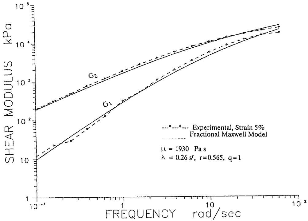
Figure 2-2 Measured Frequency Dependent Properties of Damper Fluid at 5% Strain and Comparison to Predictions of Fractional Maxwell Model.
