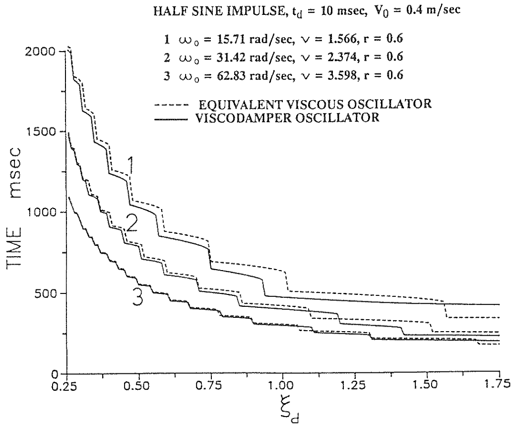
Figure 4-7 Time Needed for Displacement Response to Impulsive Loading to Reduce to Five Percent of Peak Value.
