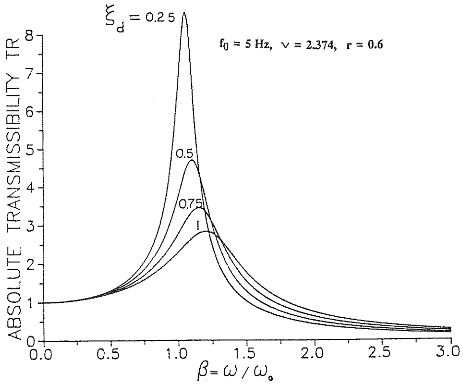
Figure 4-5 Absolute Transmissibility Plot of Viscodamper Oscillator for Steady-State Harmonic Motion.
