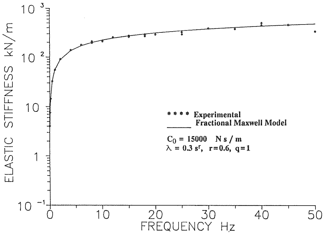
Figure 2-8 Fitting of Elastic Stiffness of Tested Damper in Vertical Motion by Fractional Maxwell Model.
