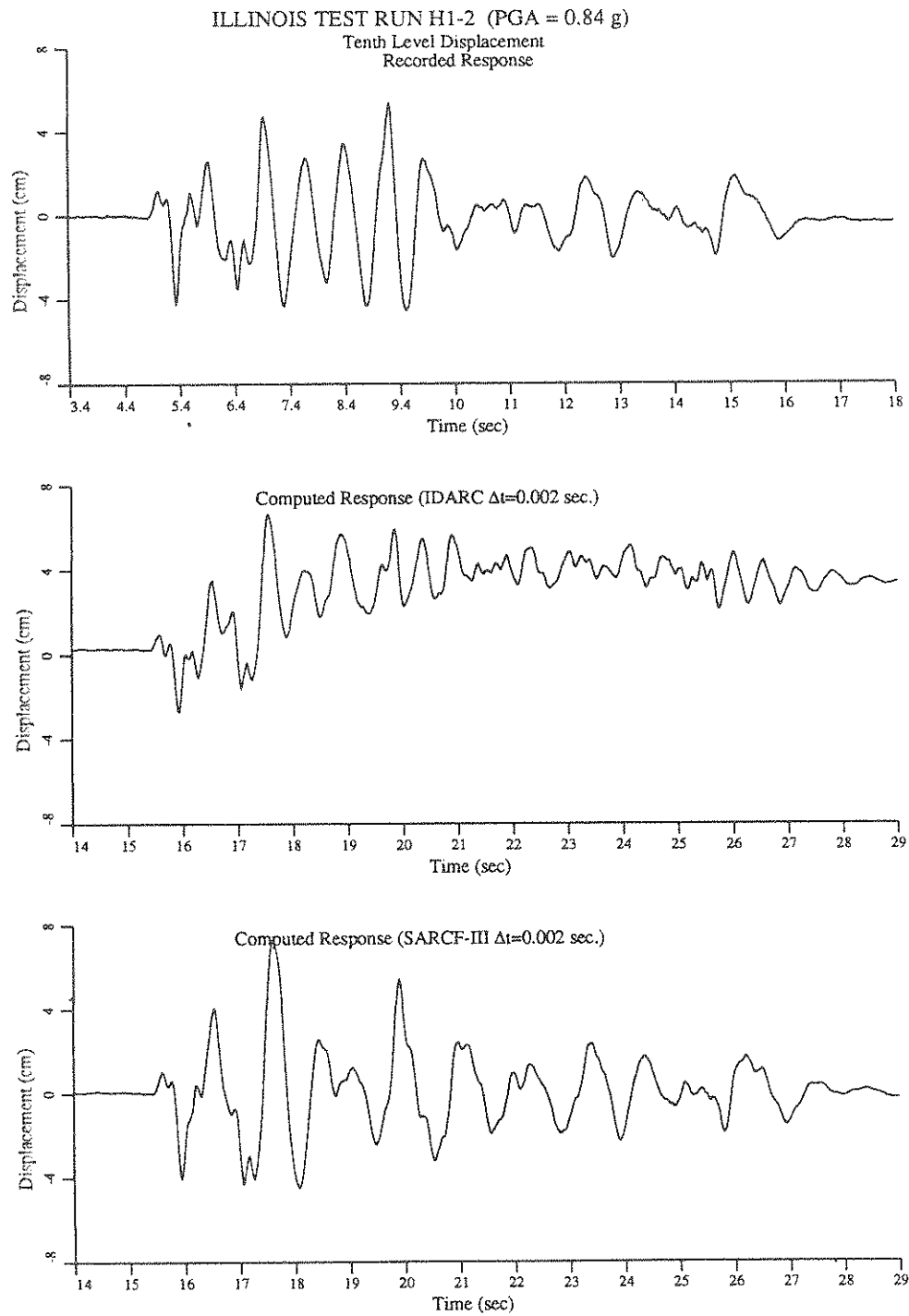
FIGURE 3-6 Comparison between Experimental and Computed Results (Second Run)
