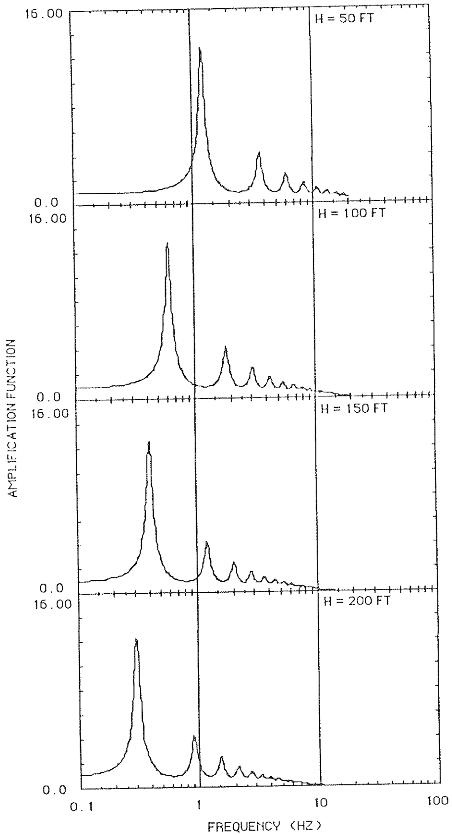
FIGURE 4-9 AMPLIFICATION FUNCTIONS ALONG THE FLUSHING LINE AT THE SUNNYSIDE SECTION (FOR 5% SOIL DAMPING)
