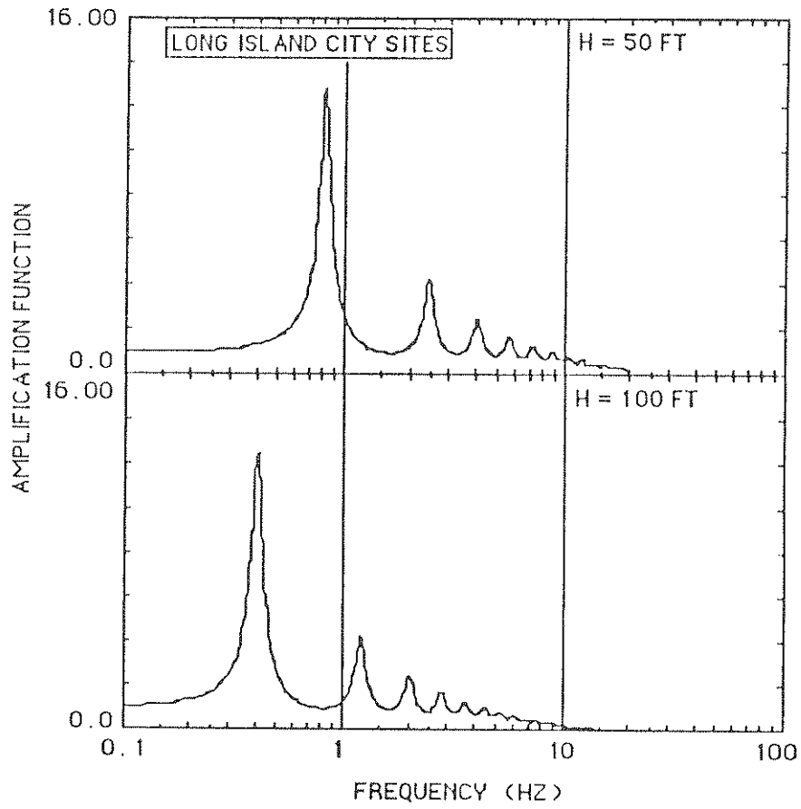
FIGURE 4-8 AMPLIFICATION FUNCTIONS ALONG THE FLUSHING LINE AT THE LIC SECTION (FOR 5% SOIL DAMPING)
