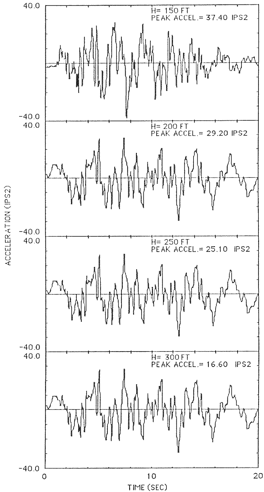
FIGURE 4-14 SURFACE ACCELEROGRAMS ALONG THE FLUSHING LINE AT THE JACKSON HEIGHTS SECTION (FOR 5% SOIL DAMPING)
