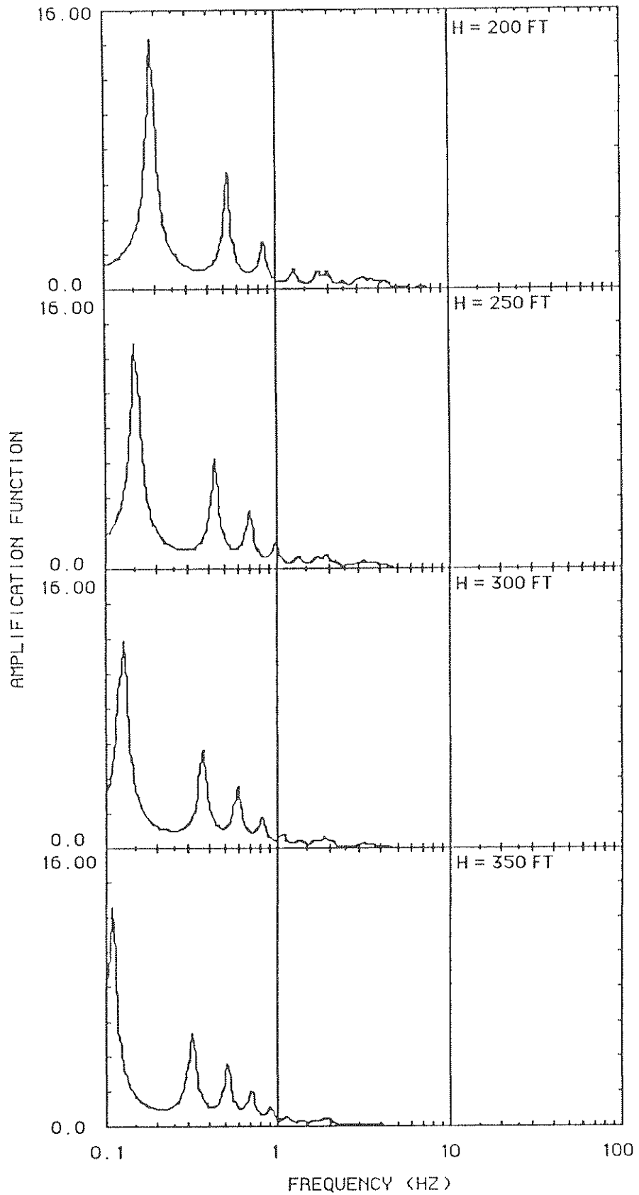
FIGURE 4-11 AMPLIFICATION FUNCTIONS ALONG THE FLUSHING LINE AT THE WILLETS POINT SECTION (FOR 5% SAND AND 2% CLAY DAMPING)
