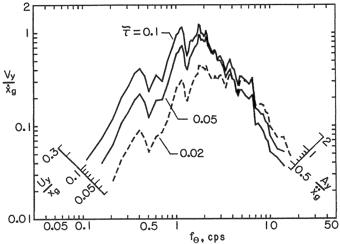
FIG. 5-5 Response Spectra for Lateral and Circumferential Structural Deformations of Systems with \zeta_x = \zeta_\theta = 0.02 Subjected to E1 Centro Free-Field Ground Motion; No Inertial Interaction
