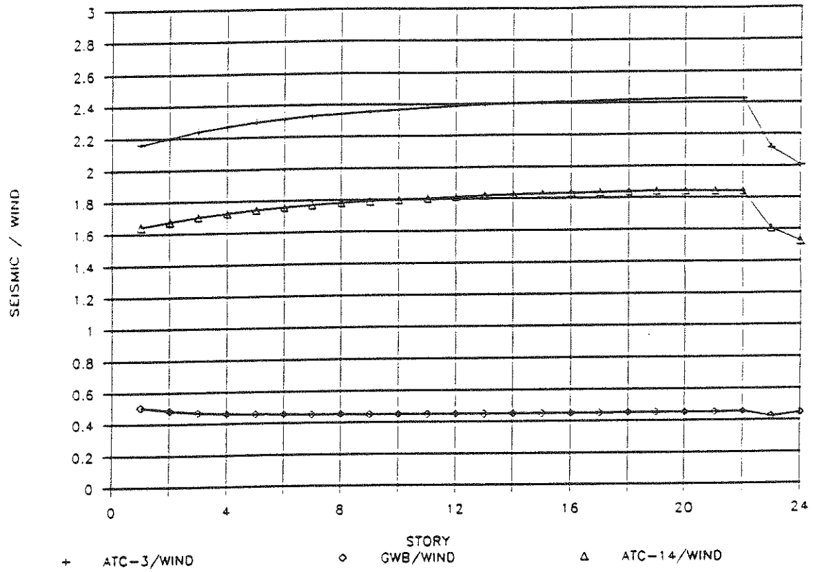
Fig. 2-16 Normalized Displacements, NY2, Y-Direction
