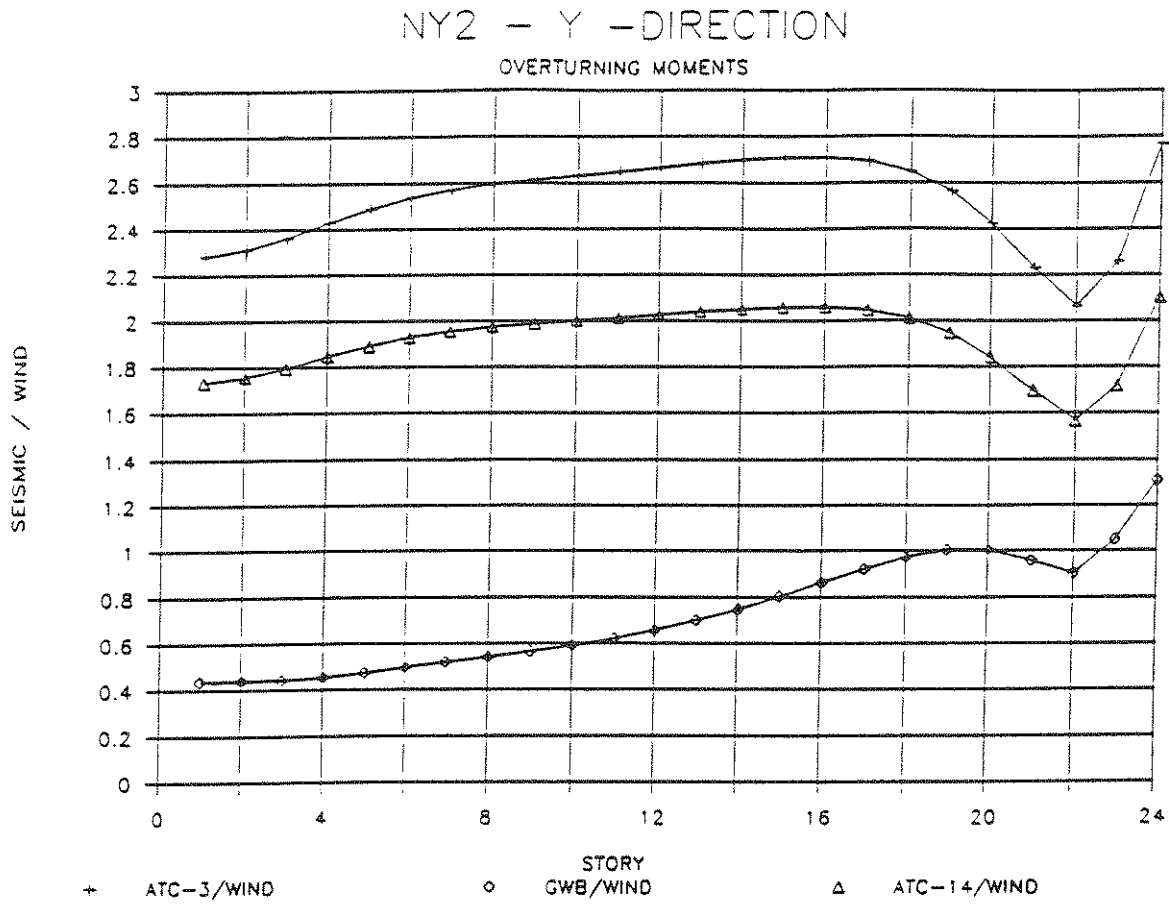
Fig. 2-18 Normalized OTM, NY2, Y-Direction
