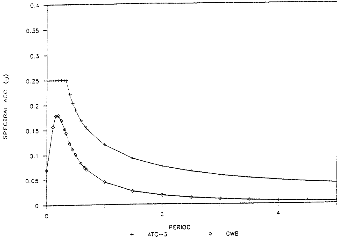
Fig. 2-4 Design Spectra
