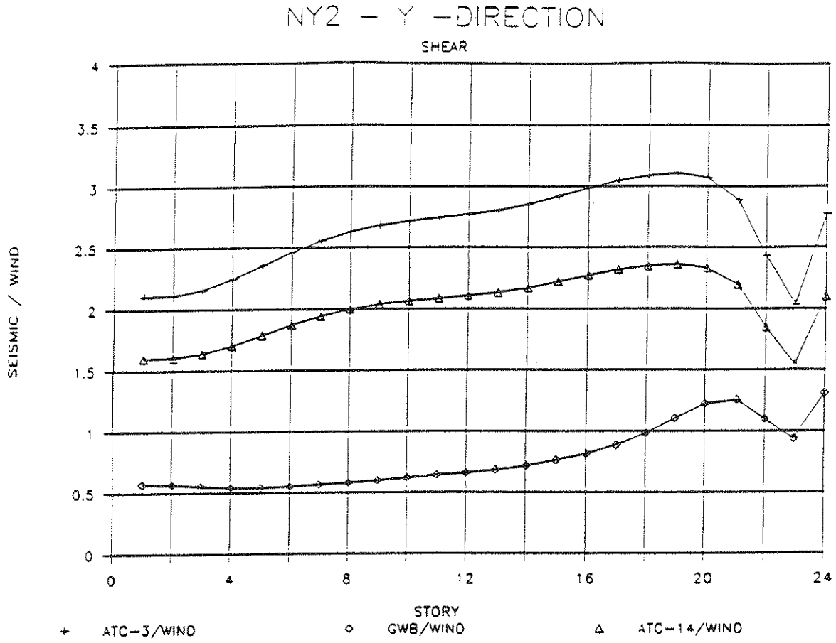
Fig. 2-17 Normalized Shear, NY2, Y-Direction
