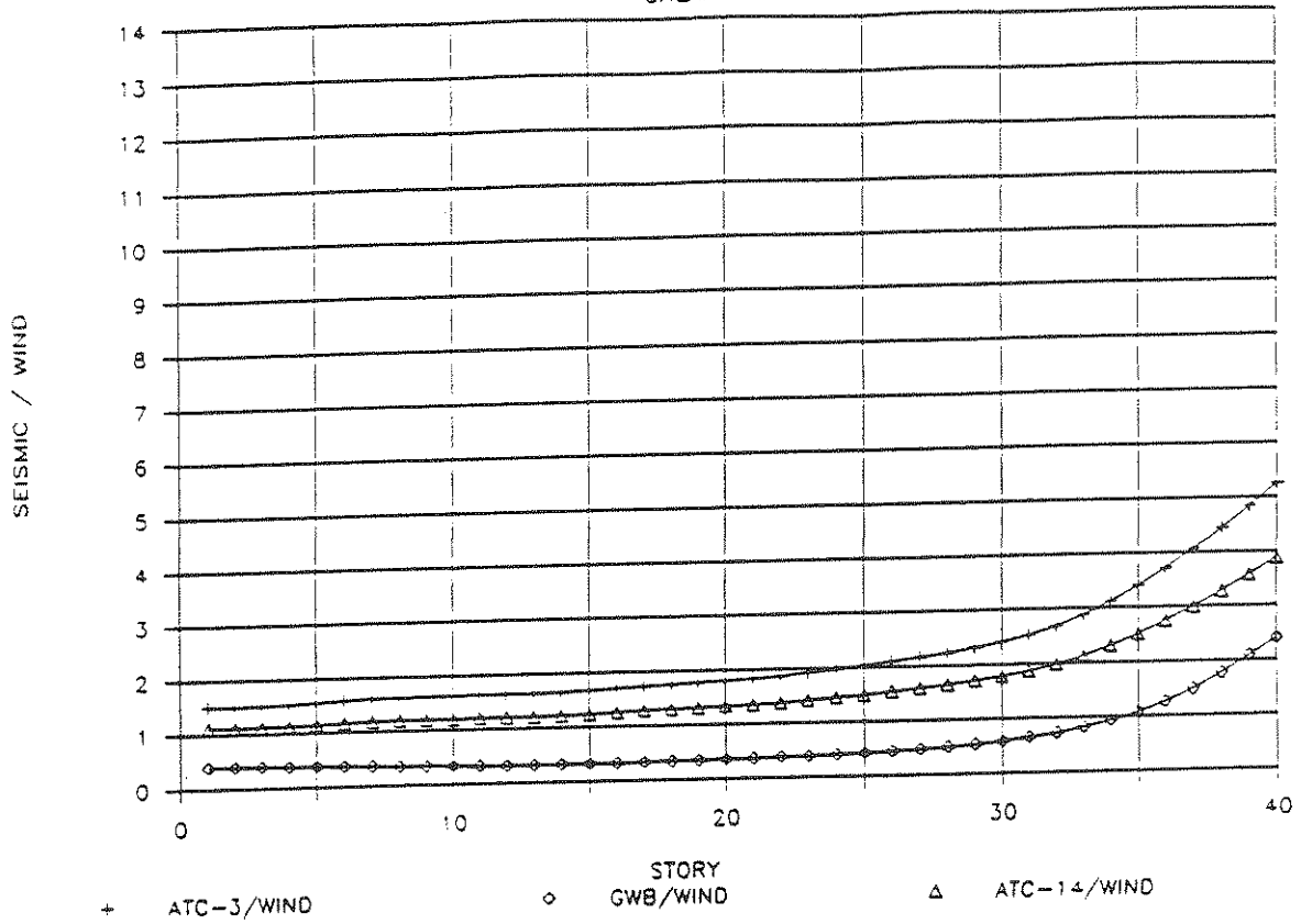
Fig. 2-11 Normalized Shear, NY1, Y-Direction
