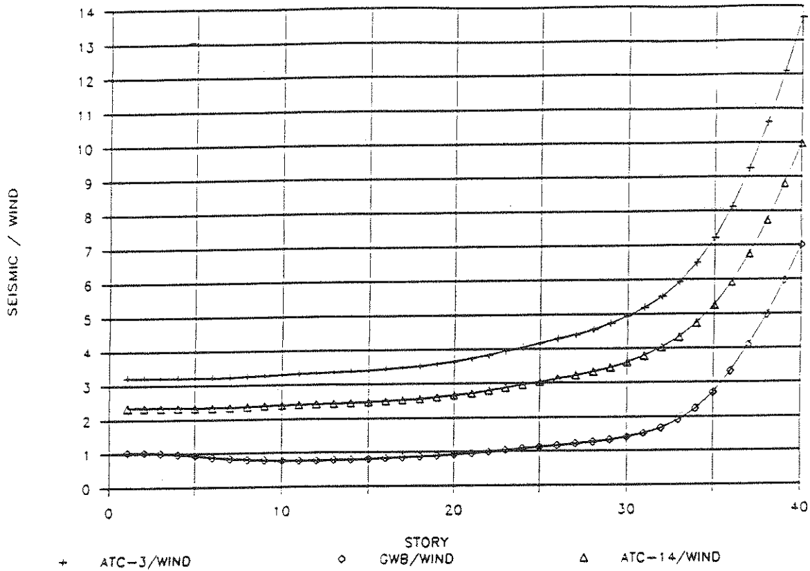
Fig. 2-8 Normalized Shear, NY1, X-Direction
