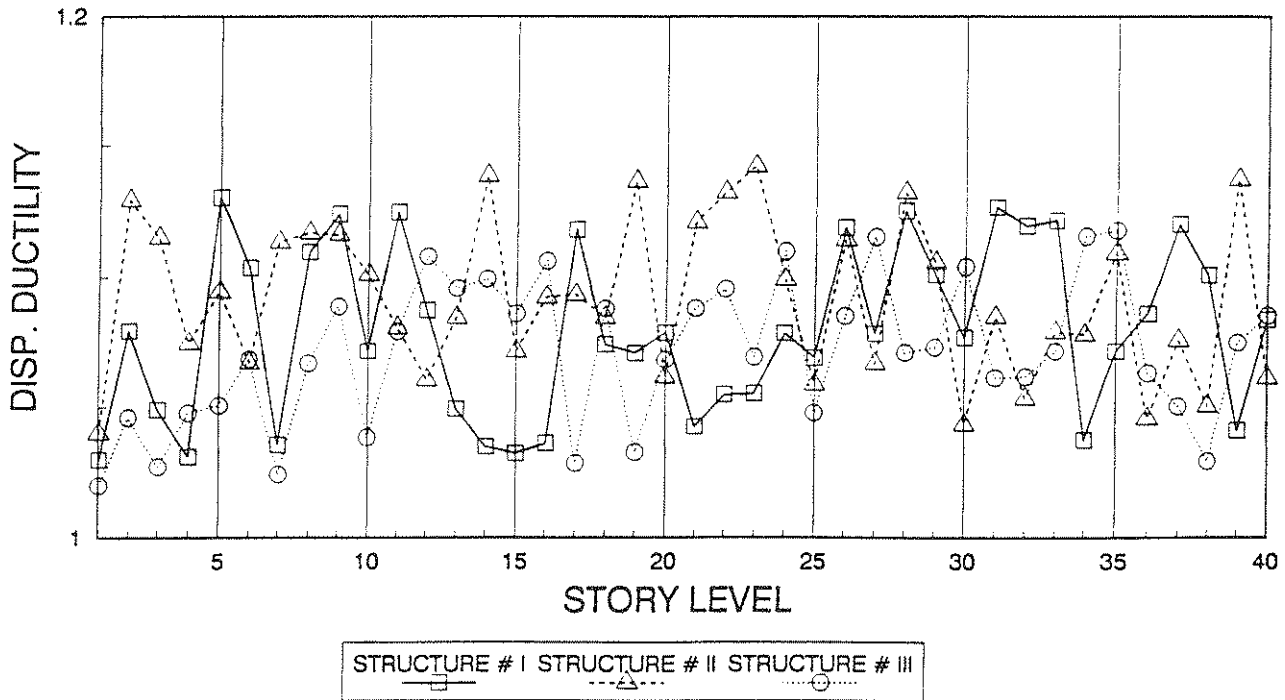
Fig. 4-6 Displacement Ductility, NY1
