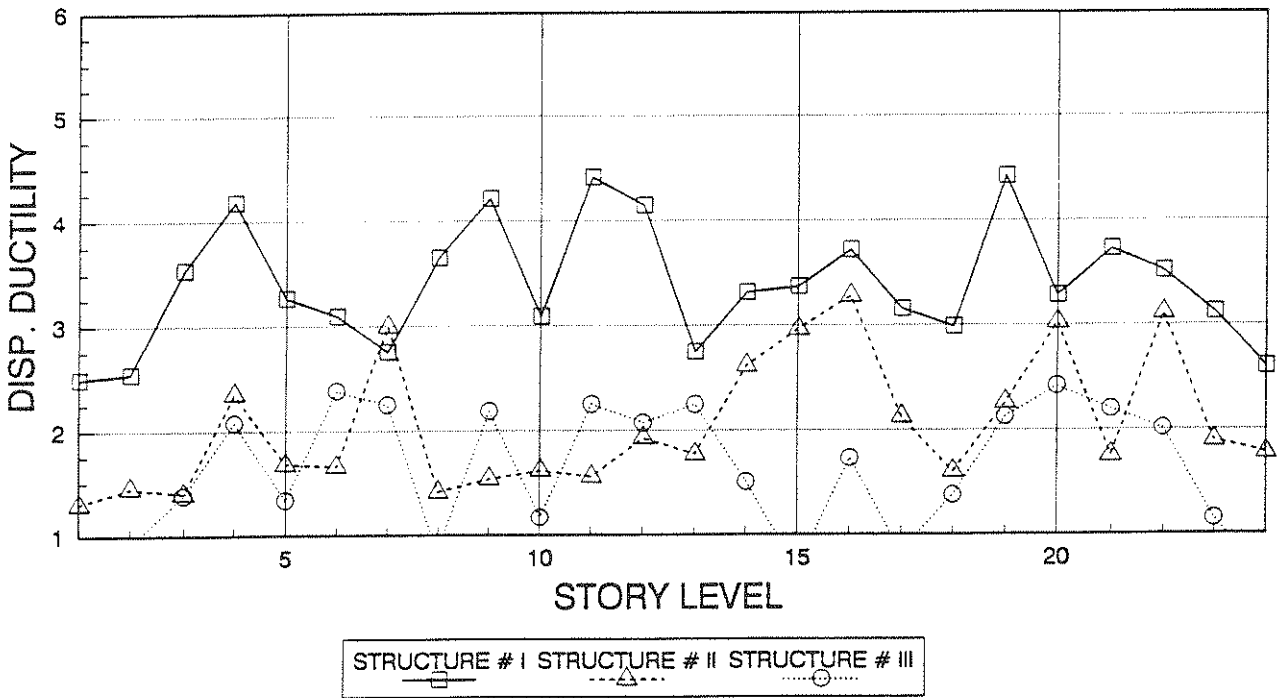
Fig. 4-5 Inter-Story Ductility, NY2
