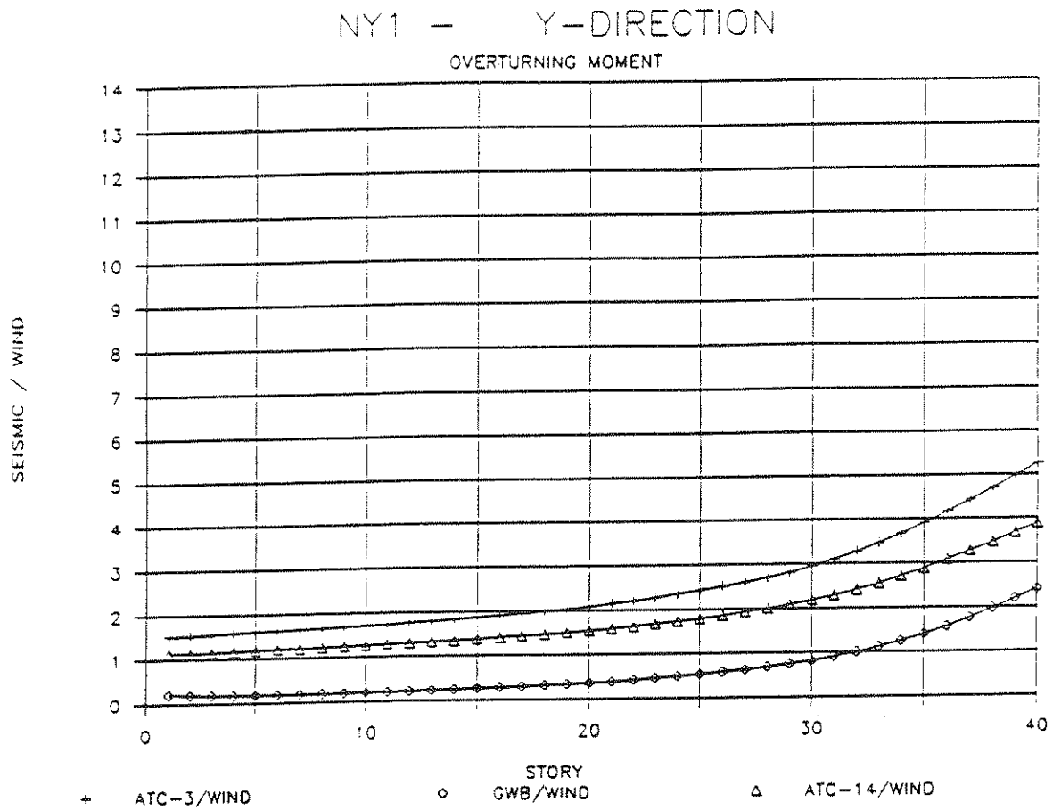
Fig. 2-12 Normalized OTM, NY1, Y-Direction
