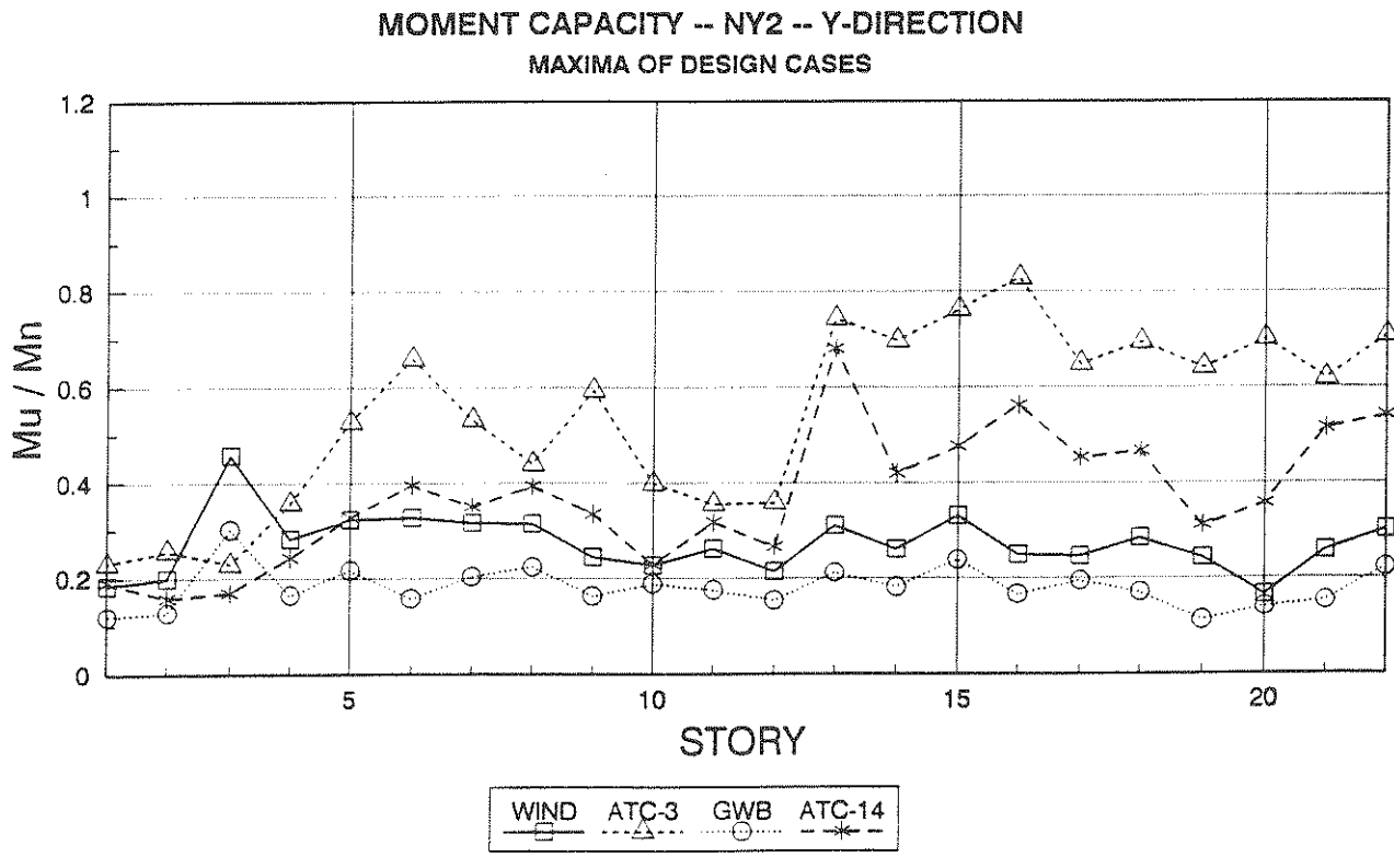
Fig. 3-4 OTM Capacity Ratio, NY2
