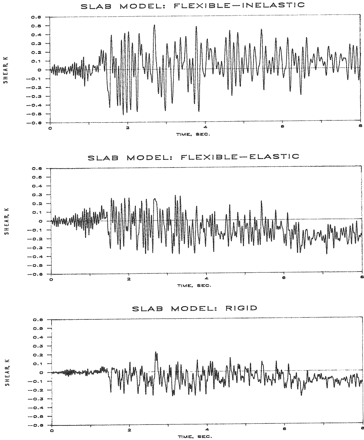
FIGURE 6-9 Base Shear Force Of the Middle Frame for the Scaled Model Structure
