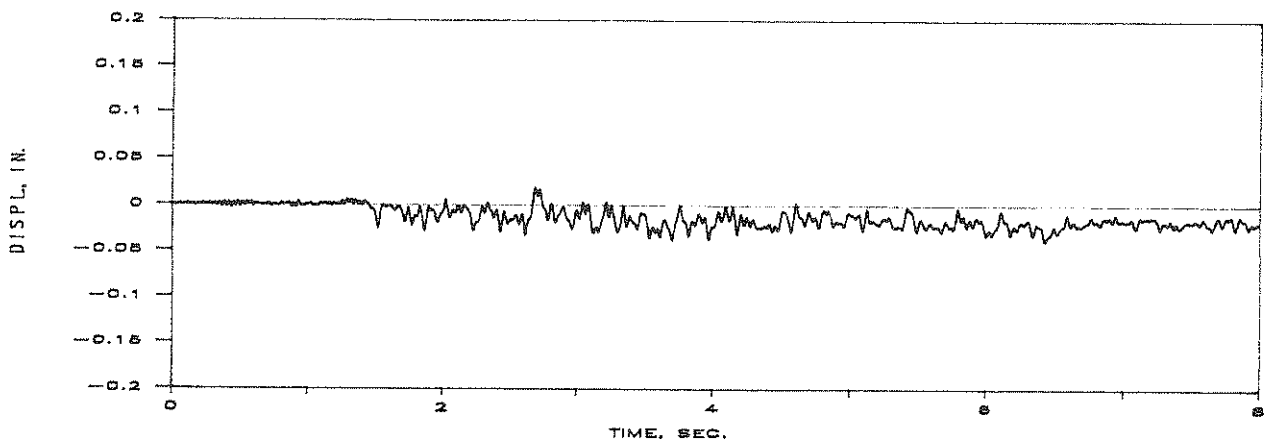
FIGURE 6-10 Lateral Displacement at the End Frame for the Scaled Model Structure
