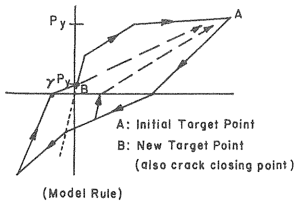
(c) Bond-Slip
