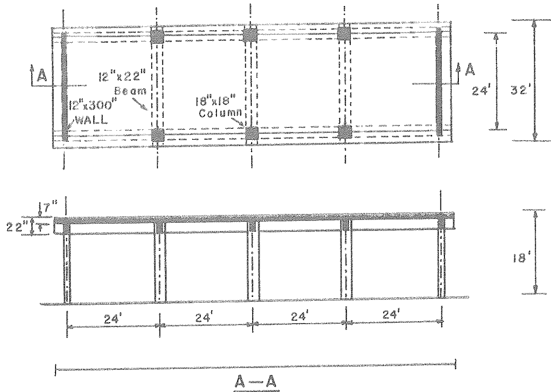
(a) Overall Geometry
