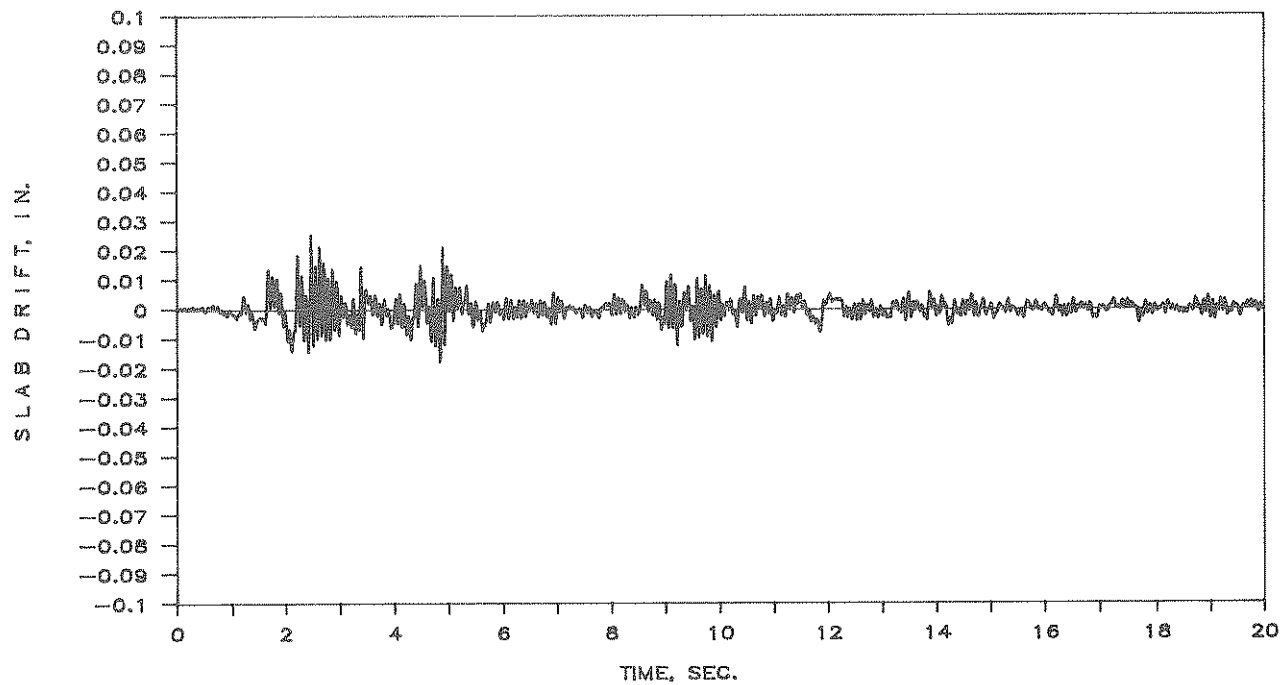
FIGURE 5-7 The Relative Displacement Between The Middle Frame and the End Wall (Slab Drift) for 4 Span Structure
