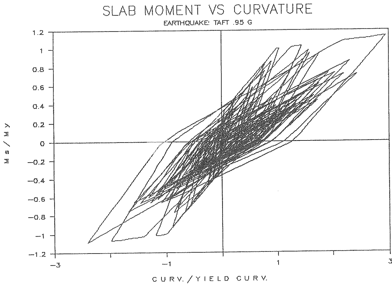
FIGURE 6-7b Moment-Curvature Plot at Mid-region of the interior panel for the Scaled Model Structure
