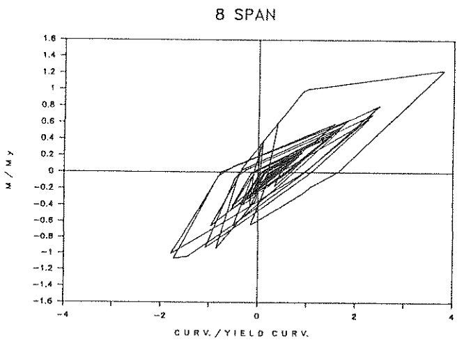
FIGURE 5-12 Slab Moment-Curvature Curves for the Multi-Span Structure Using Inelastic Slab Models
