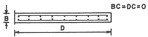
PLAN B-B
