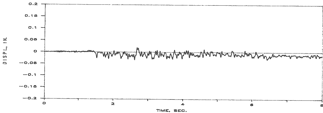
FIGURE 6-8 Lateral Displacement at Middle Frame for the Scaled Model Structure
