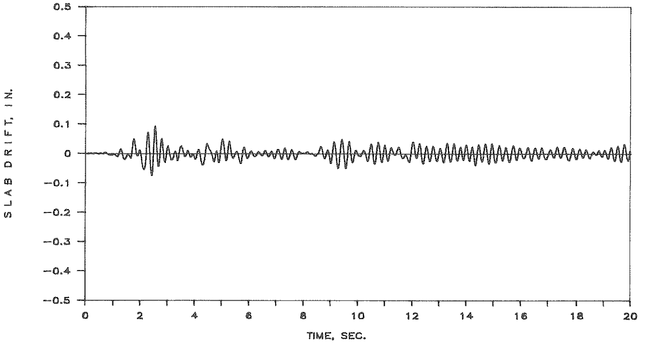
FIGURE 5-9 The Relative Displacement Between The Middle Frame and the End Wall (Slab Drift) for 8 Span Structure
