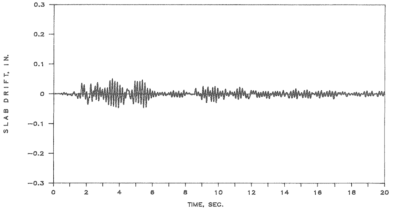
FIGURE 5-8 The Relative Displacement Between The Middle Frame and the End Wall (Slab Drift) for 6 Span Structure
