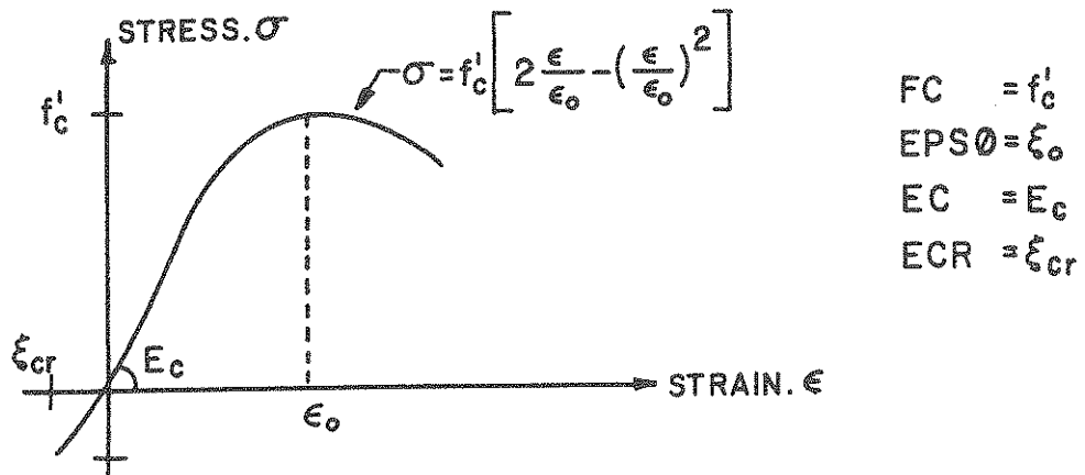
FIGURE A-3 Concrete Stress-Strain Curve
