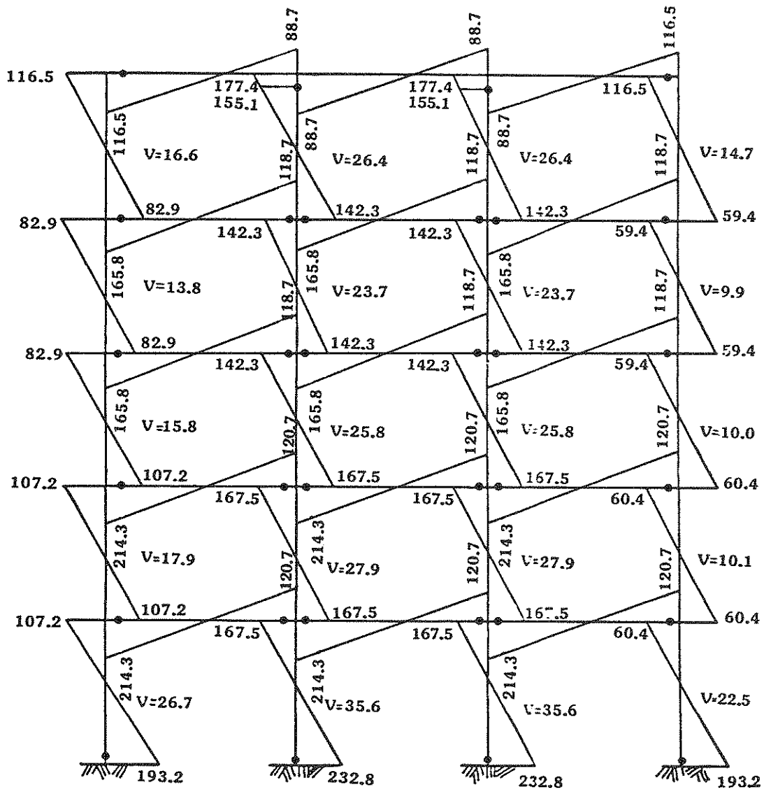
Fig. 7-5 Failure Mechanism and Moment Distribution (Case1)
