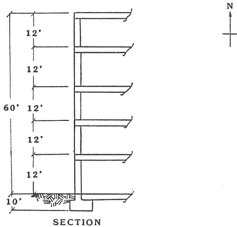
Fig. B-1 Five-Story Frame Structure
