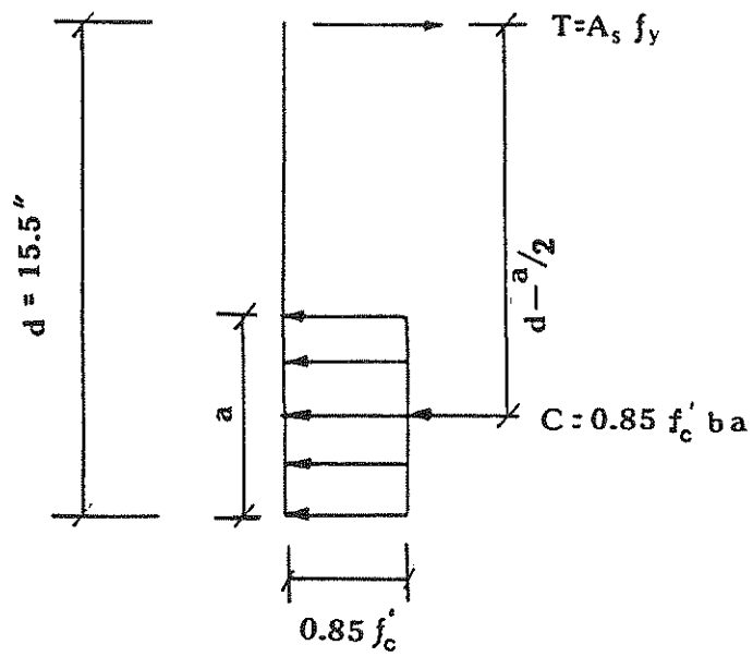
Fig. B-10 Internal Forces
