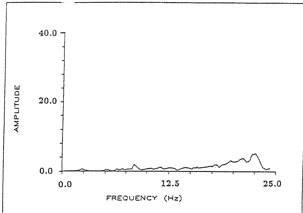
FIGURE 5-1(a) Transfer Function of Measured Acceleration to Banded White Noise Input
