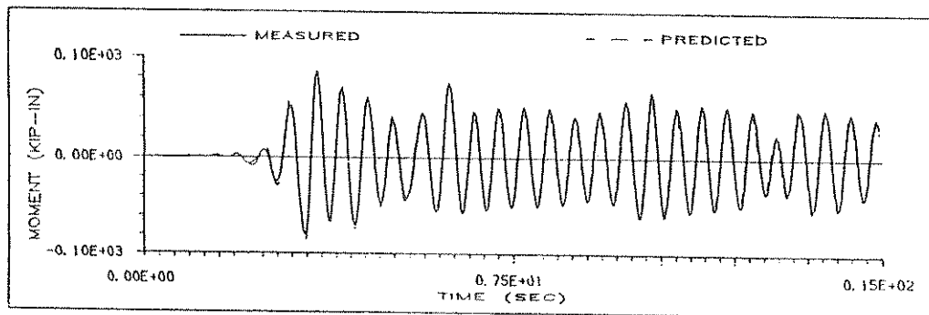
(d.2) Moment at SW Column Top
