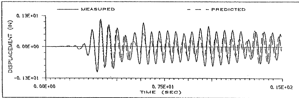
(b.1) Story Relative Displacement
