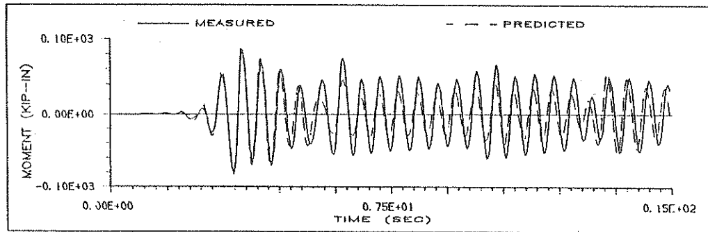
(b.2) Moment at SW Column Top
