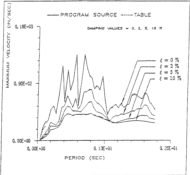
(b.3) Response Spectra
