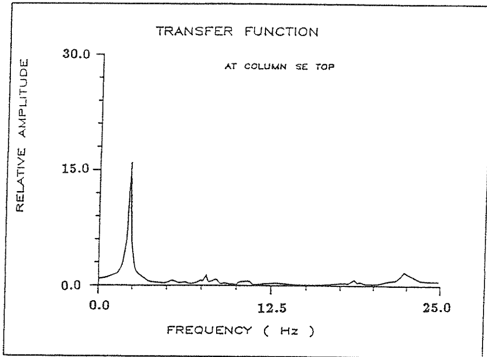
FIGURE 5-1(a) Transfer Function of Measured Acceleration to Banded White Noise Input
