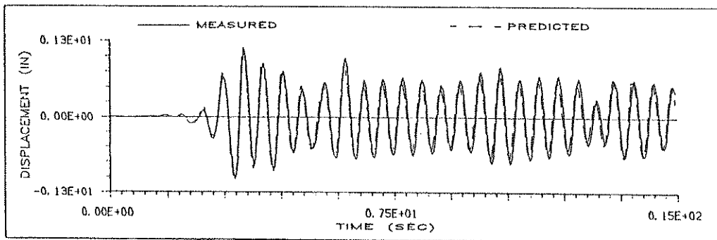
(d.1) Story Relative Displacement
