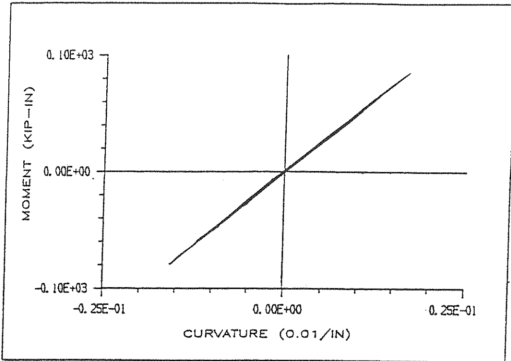
(a) at SW Column Top
