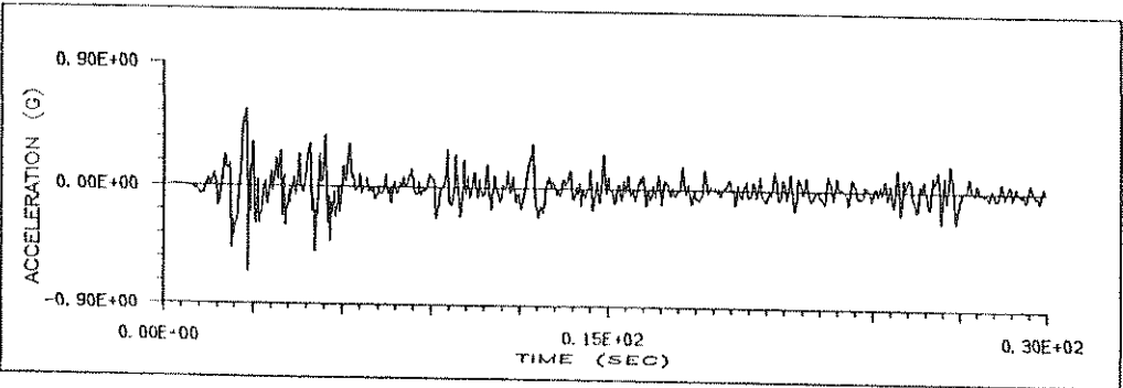
(b.2) Measured Table Acceleration
