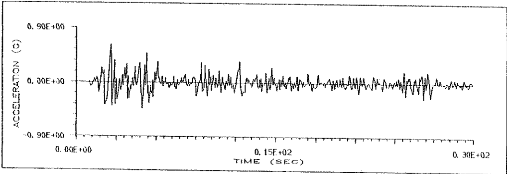
(b.1) Input Table Acceleration
