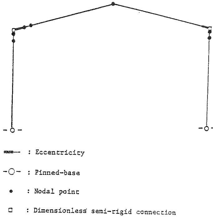
FIGURE 5-10(c) Mathematical Model 2
