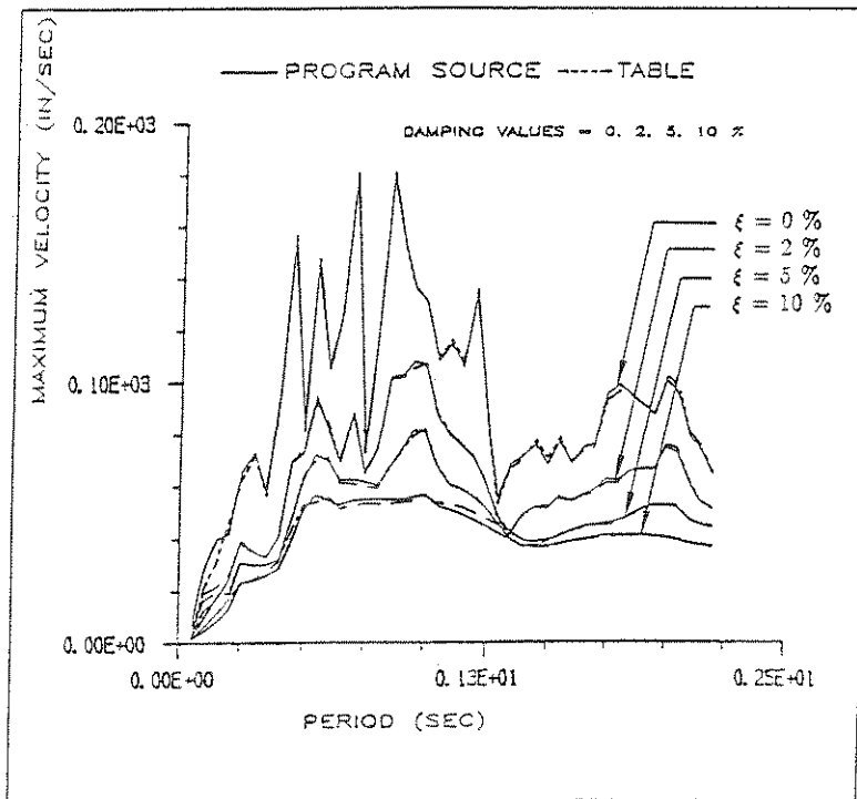
(c.3) Response Spectra
