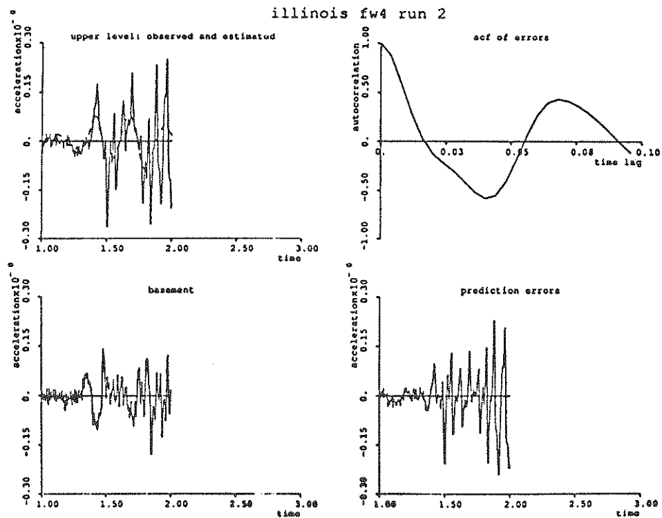
FIGURE 3-26a Example of Analysis Using a One-Mode Model
