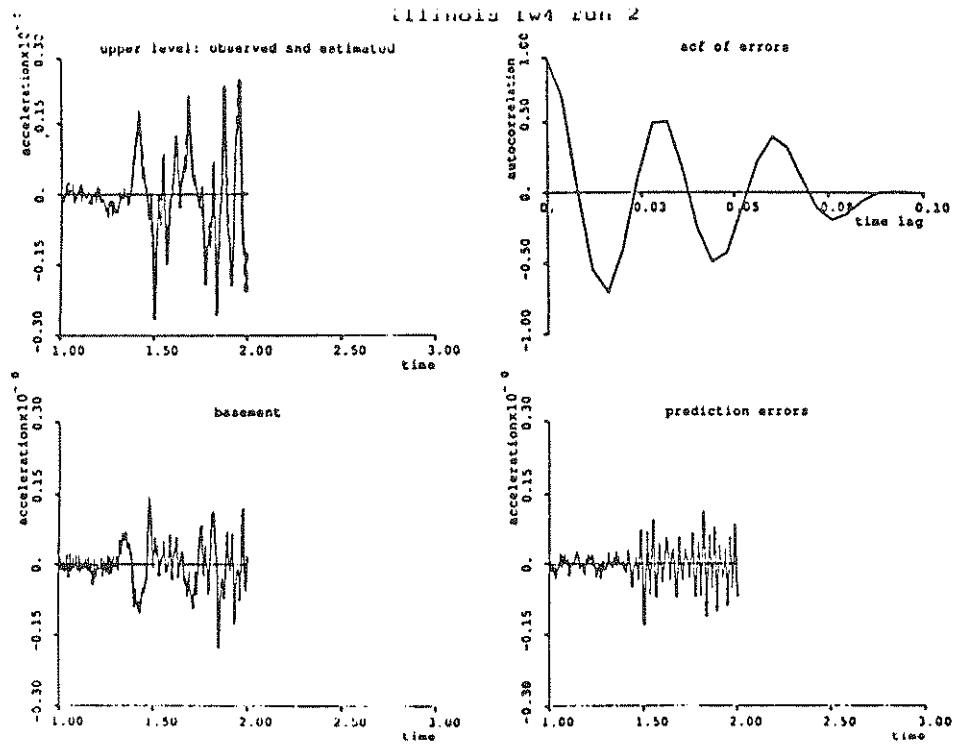
FIGURE 3-26b Example of Analysis Using a Two-Mode Model
