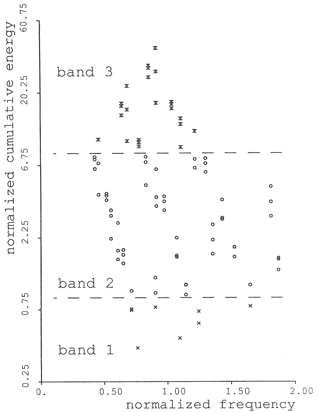
Fig. 3.12: Normalized Frequency and Cumulative Energy for the Earthquakes Simulated
