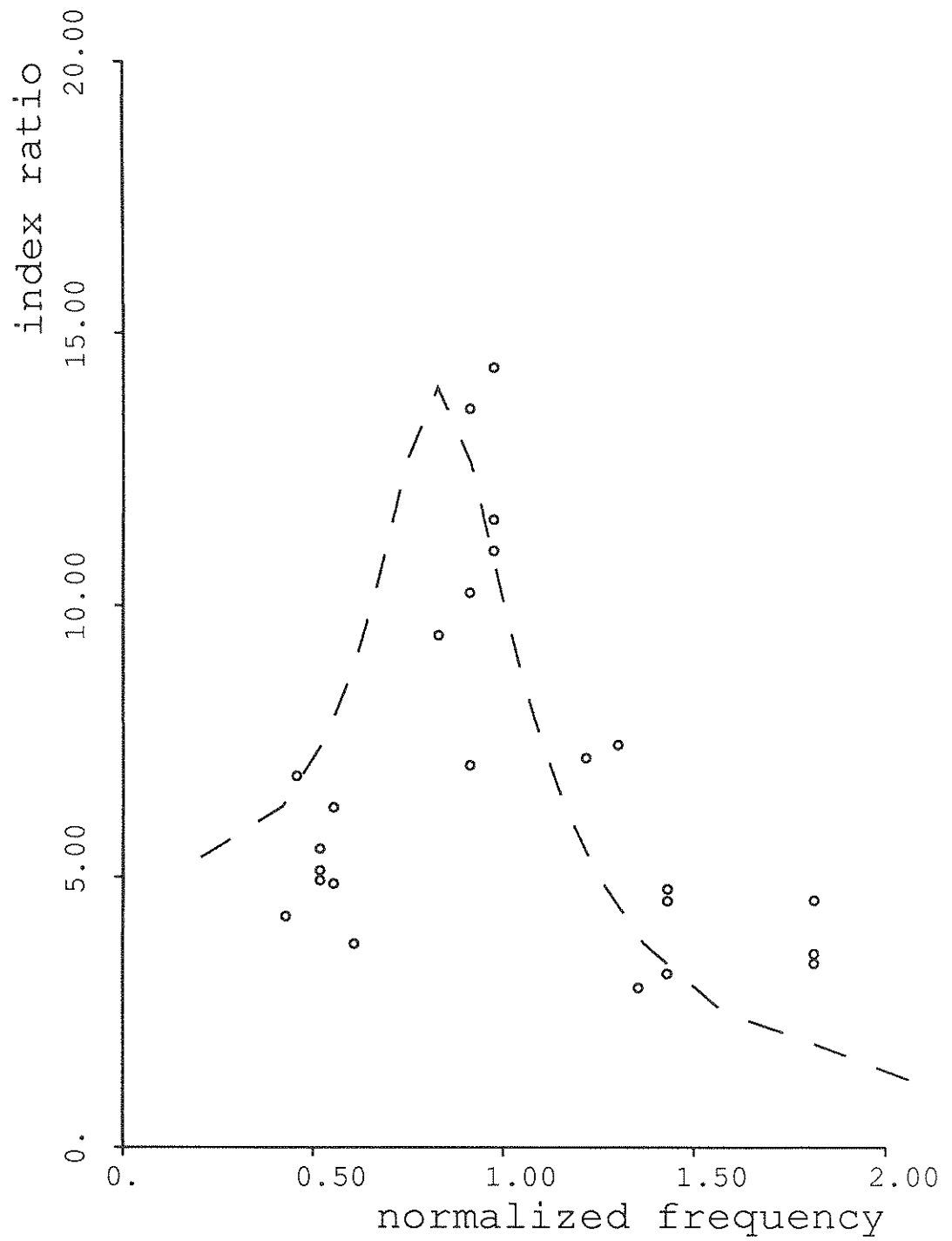
Fig. 3.14: Index Ratio vs. Normalized Frequency: Intermediate Cumulative Energy
