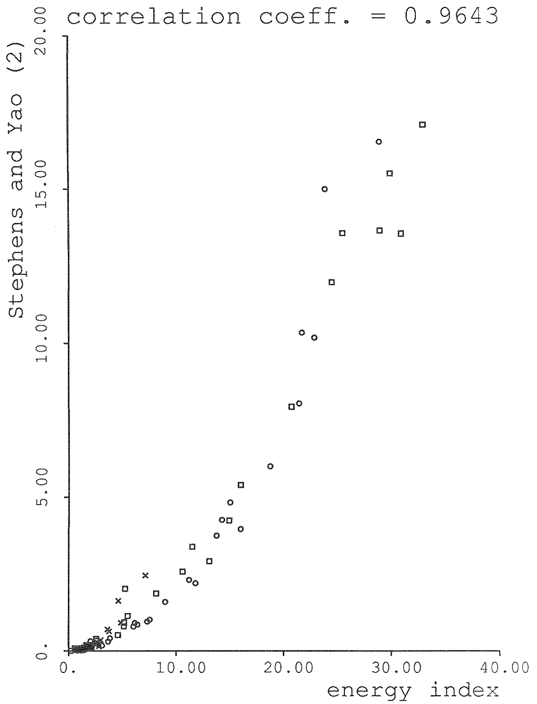
fig.3.8: Energy Index vs. Stephens' Index
