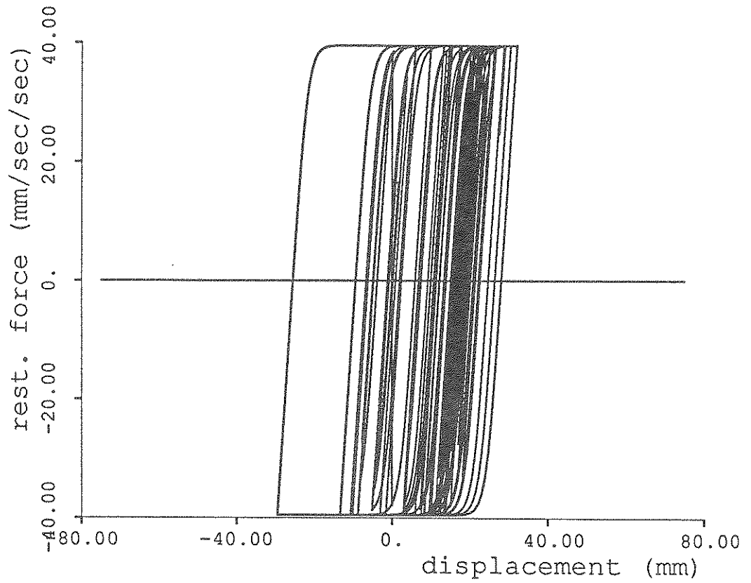
Fig. 4.2a: Symmetric Hysteresis Cycle
