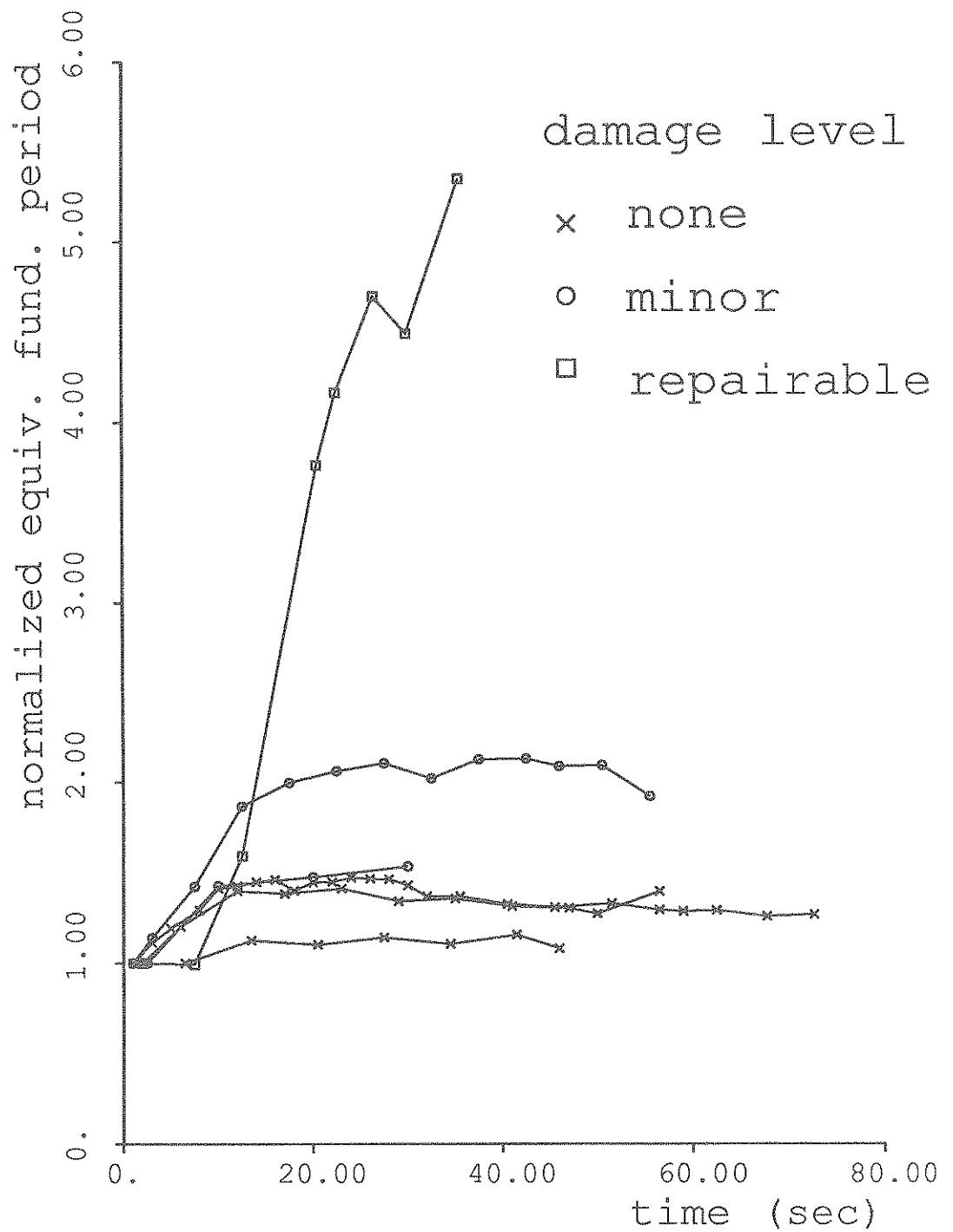
Fig. 6.6: Evolution of the Equivalent Fundamental Period
