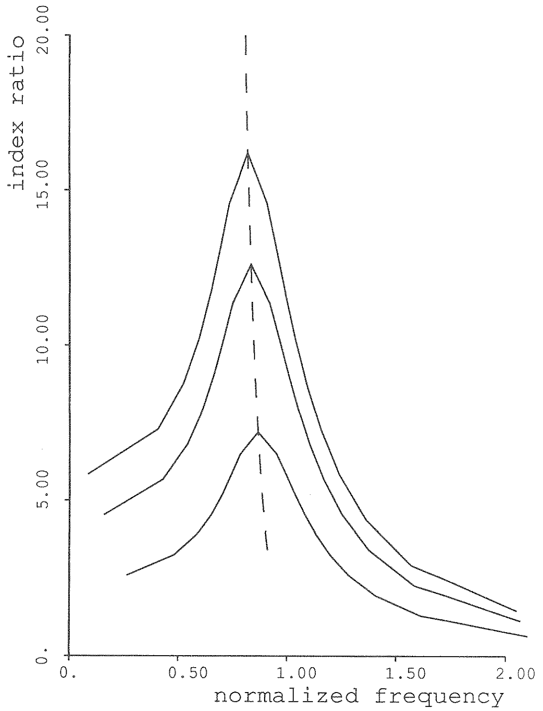
Fig. 3.16: Comparison of the Resonance Curves
