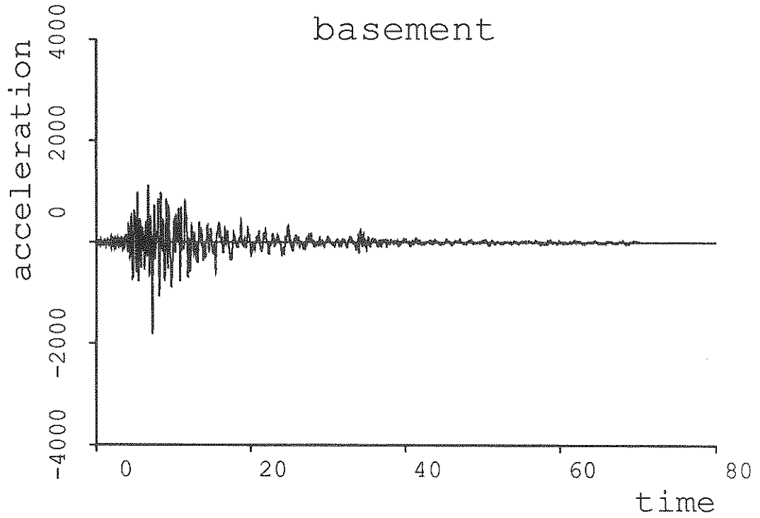
Fig. 6.1: Accelerograms from Millikan Library (EW)
