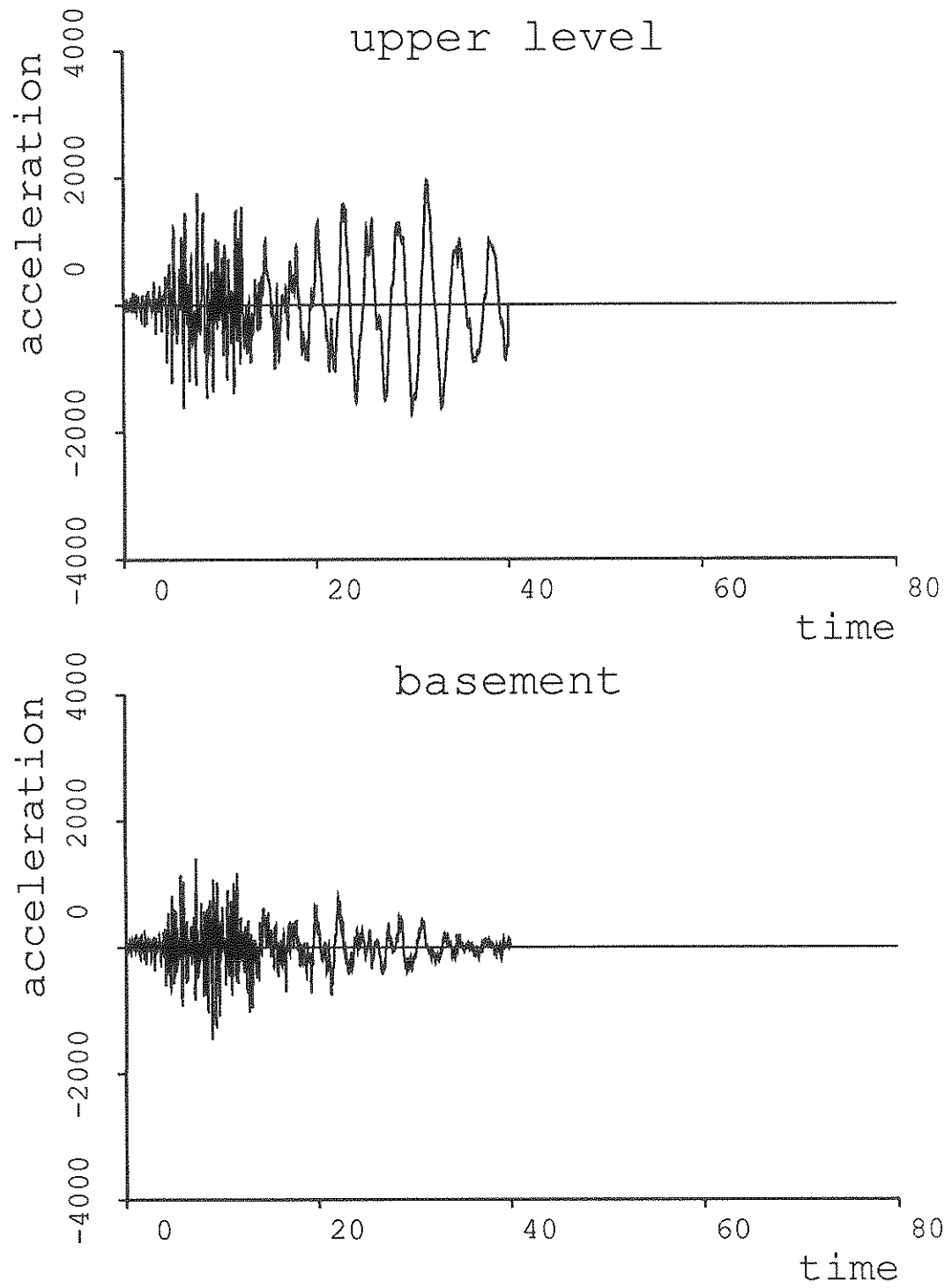
Fig. 6.5: Accelerograms from Bank of California (N79E)
