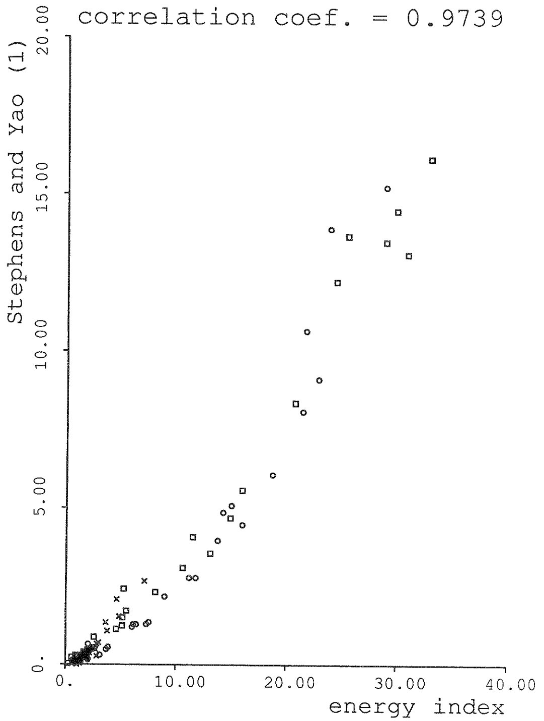
fig.3.7: Energy Index vs. Stephens' Index
