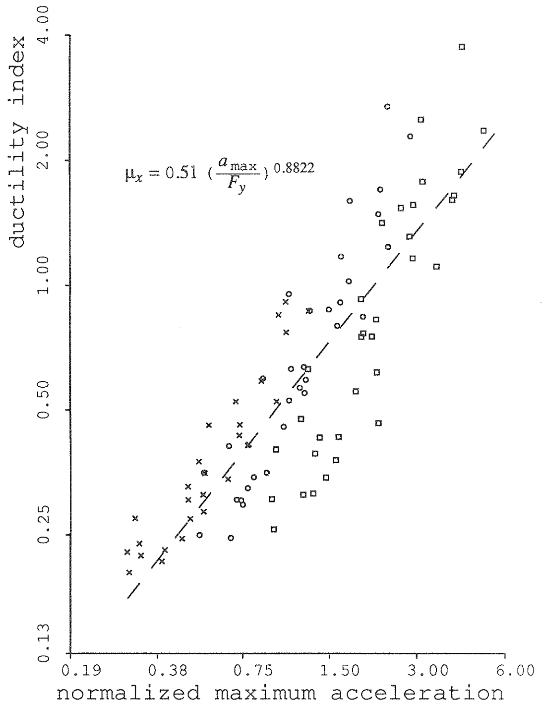
fig.3.10: Ductility Index vs. Normalized Max. Acceleration
