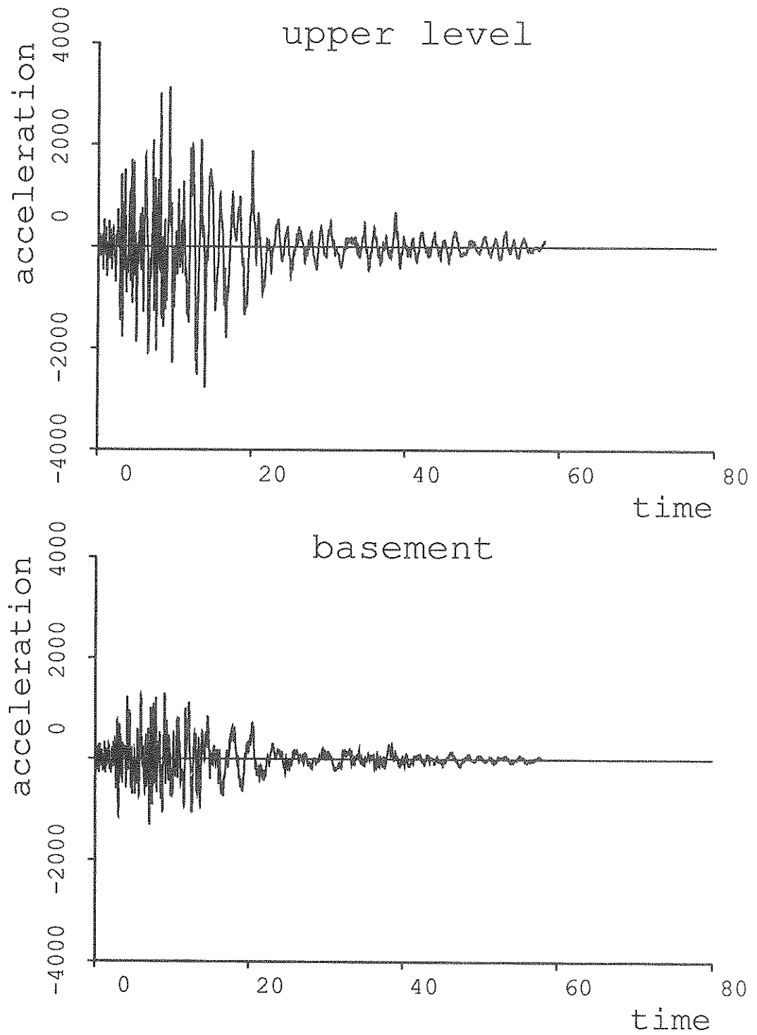
Fig. 6.4: Accelerograms from Holiday Inn Orion (S90W)
