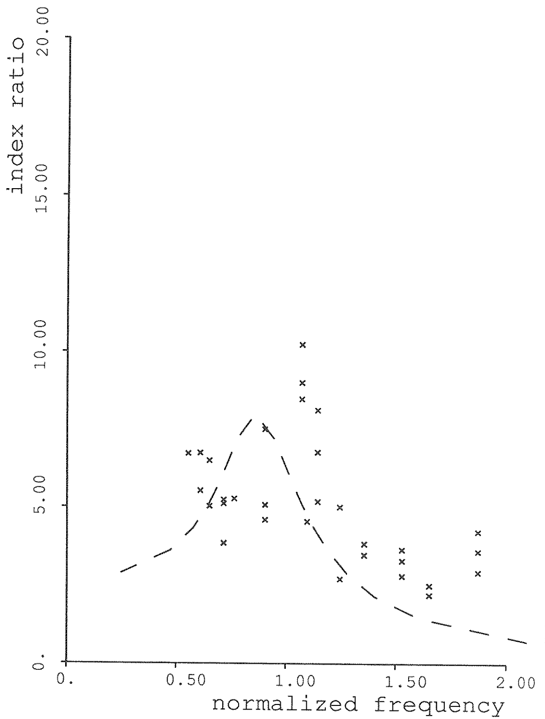
Fig. 3.13: Index Ratio vs. Normalized Frequency: low cumulative energy
