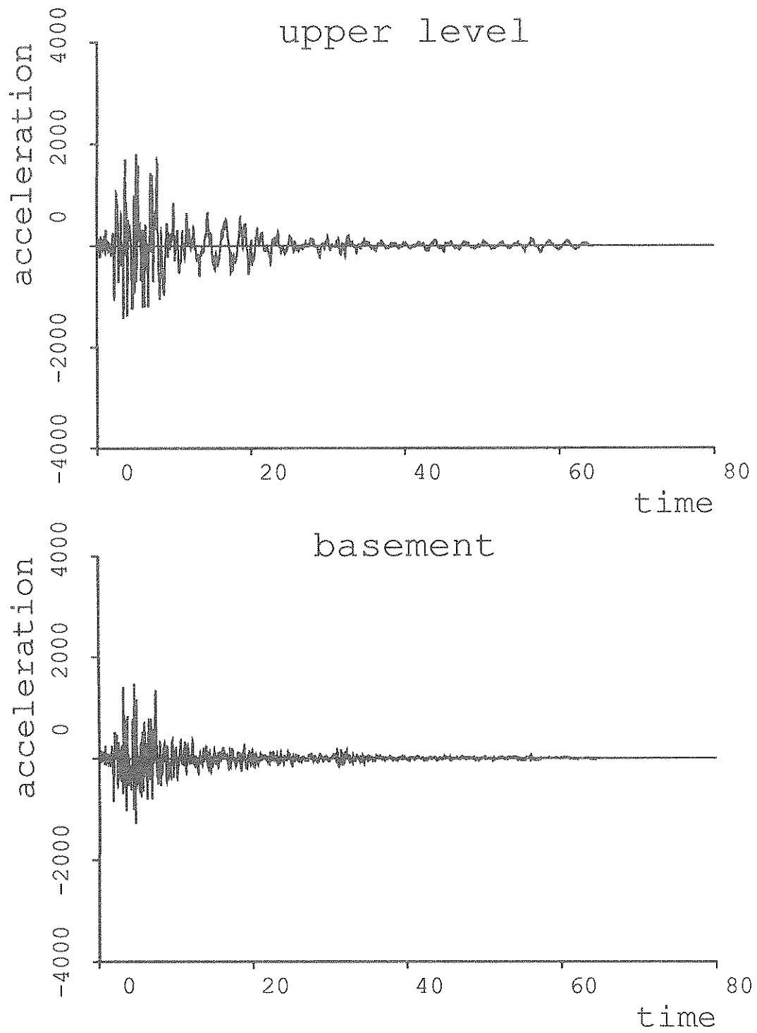
Fig. 6.3: Accelerograms from Sheraton Hotel (S90W)
