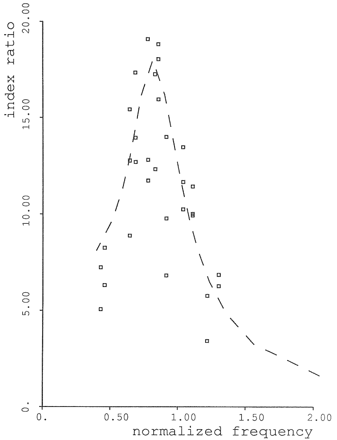
Fig. 3.15: Index Ratio vs. Normalized Frequency: High Cumulative Energy
