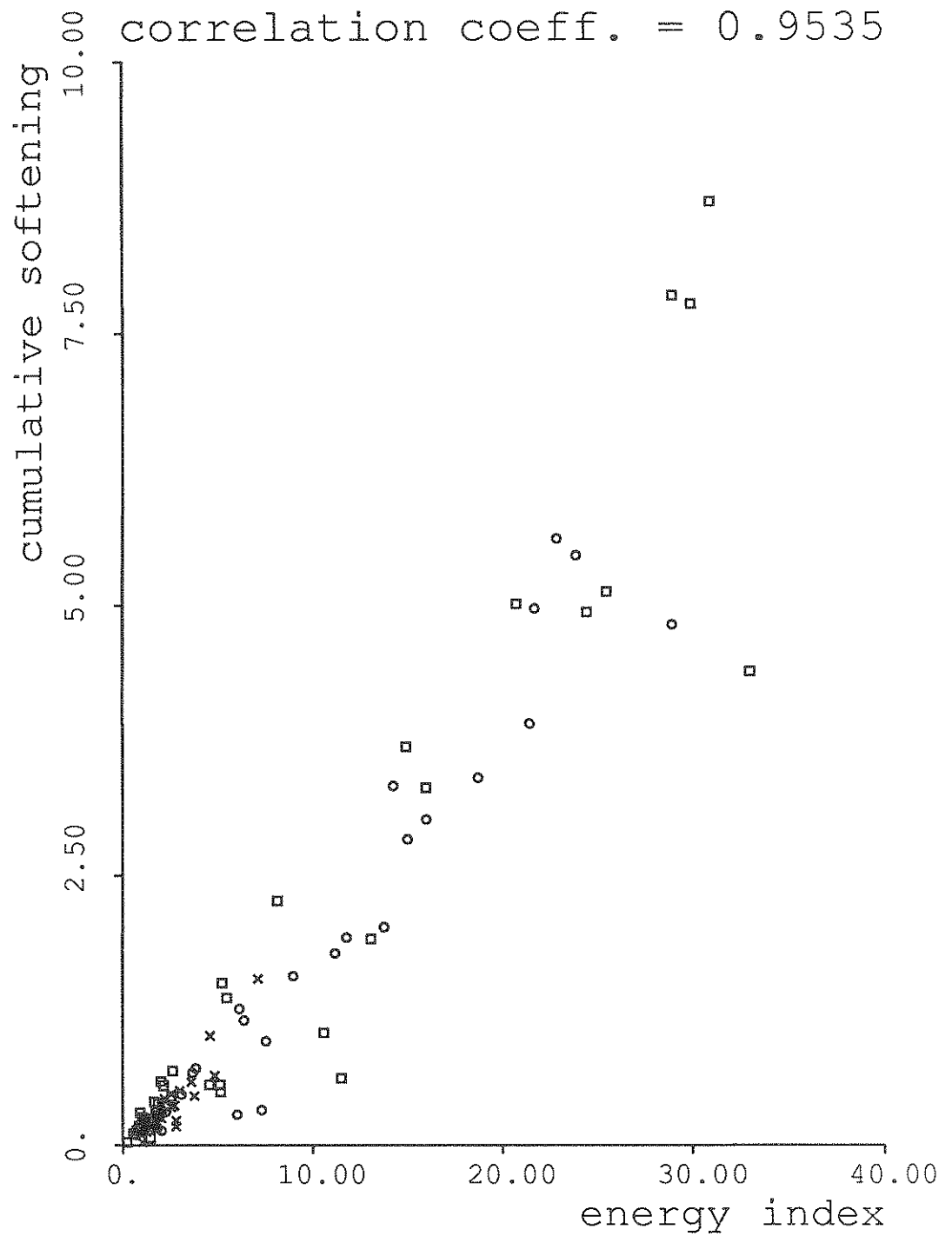
fig.4.3: Energy Index vs. Cumulative Softening
