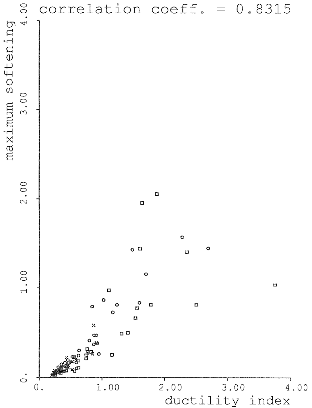
fig.4.1: Ductility Index vs. Maximum Softening
