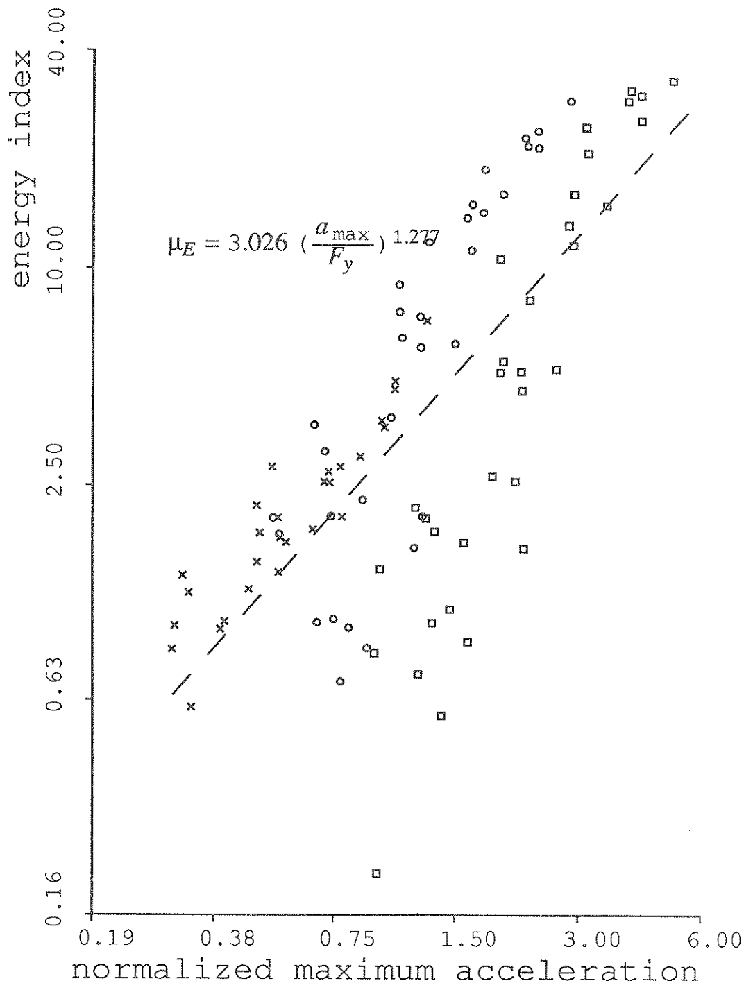
fig.3.11: Energy Index vs. Normalized Max. Acceleration
