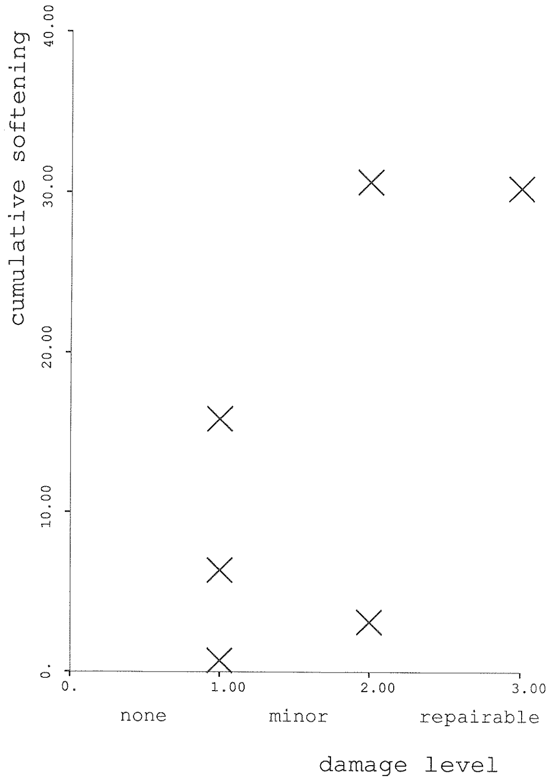
Fig. 6.8: Cumulative Softening vs. Damage Level
