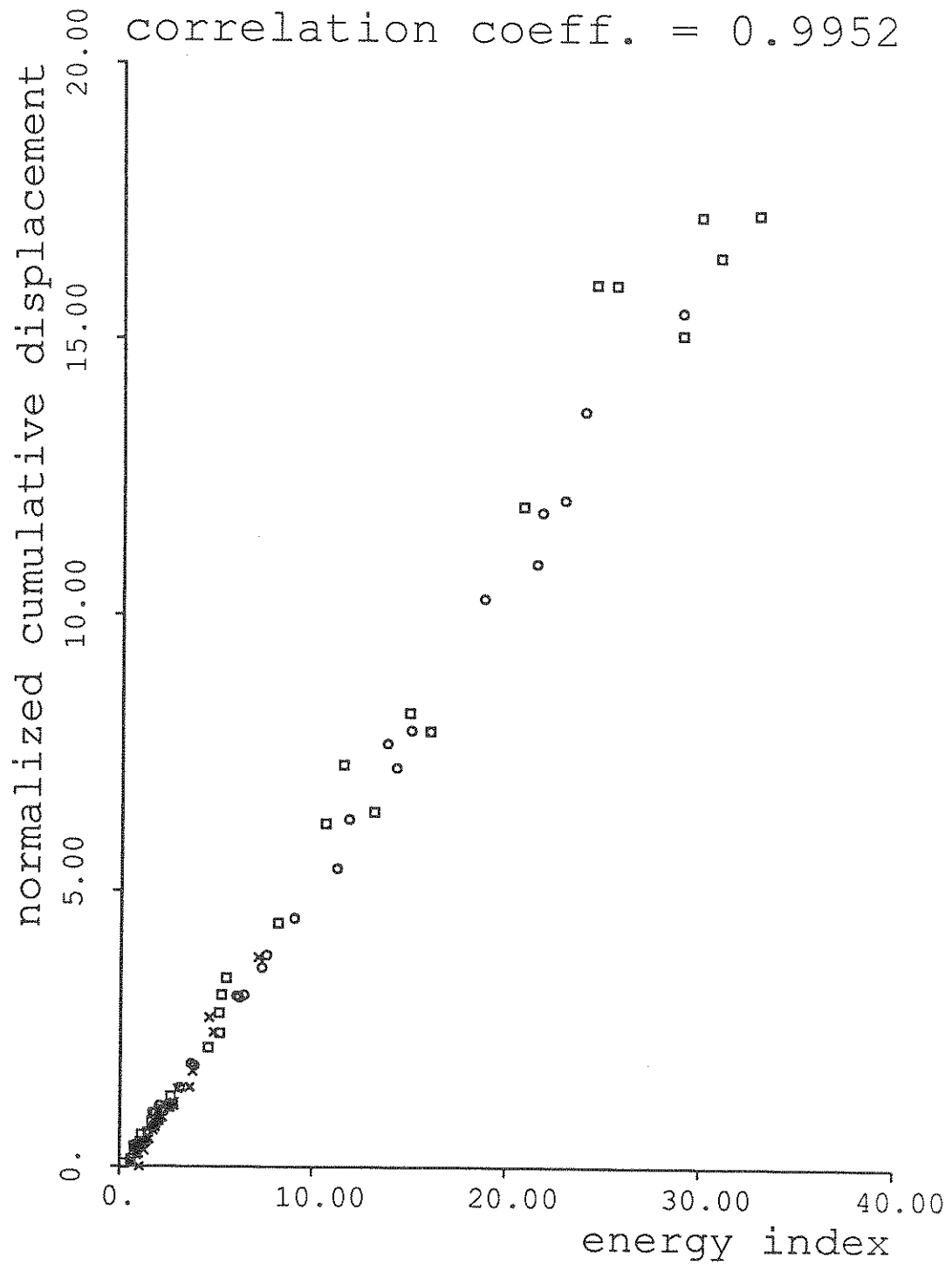
fig.3.5: Energy Index vs. Normalized Cumulative Displacement
