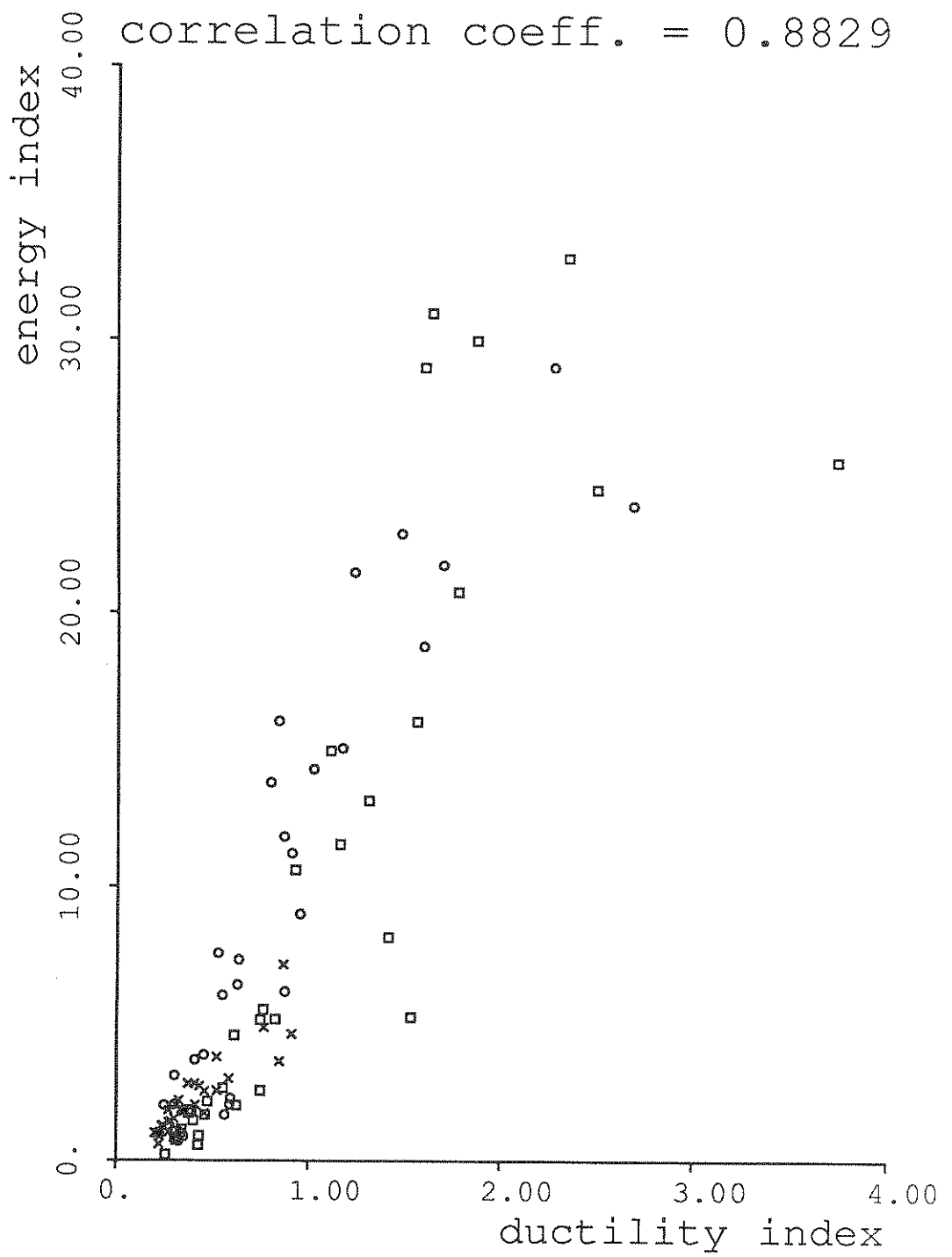
fig.3.9: Ductility Index vs. Energy Index
