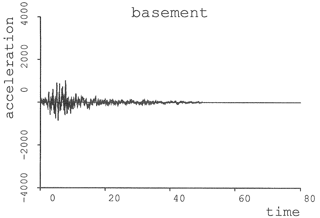
Fig. 6.2: Accelerograms from 611 West 6th St. (N38E)
