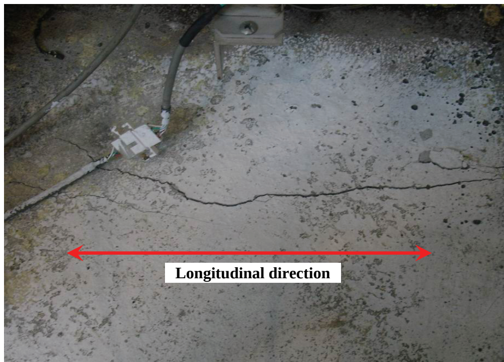
FIGURE 4-8 Onset of the Crack in Intermediate Concrete Slab (Photo Courtesy of C.H.Lin and K.C.Tsai, NCREE)
