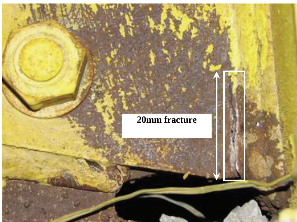
(a) Detail of the Fracture at the Shear Tab
