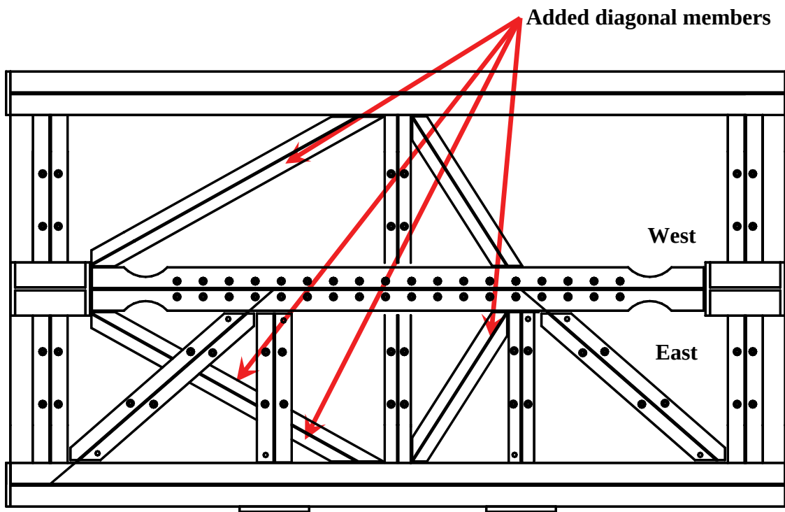
FIGURE 4-11 Layout of the Intermediate Floor Truss Strengthened after Test 1
