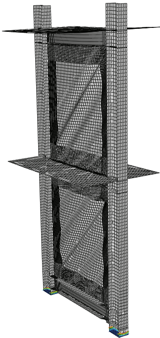
(b) Tension Field in the 3D Model
