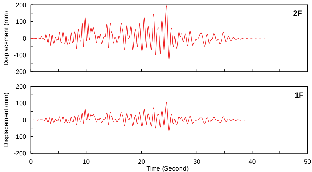
FIGURE 5-7 Displacement Inputs
