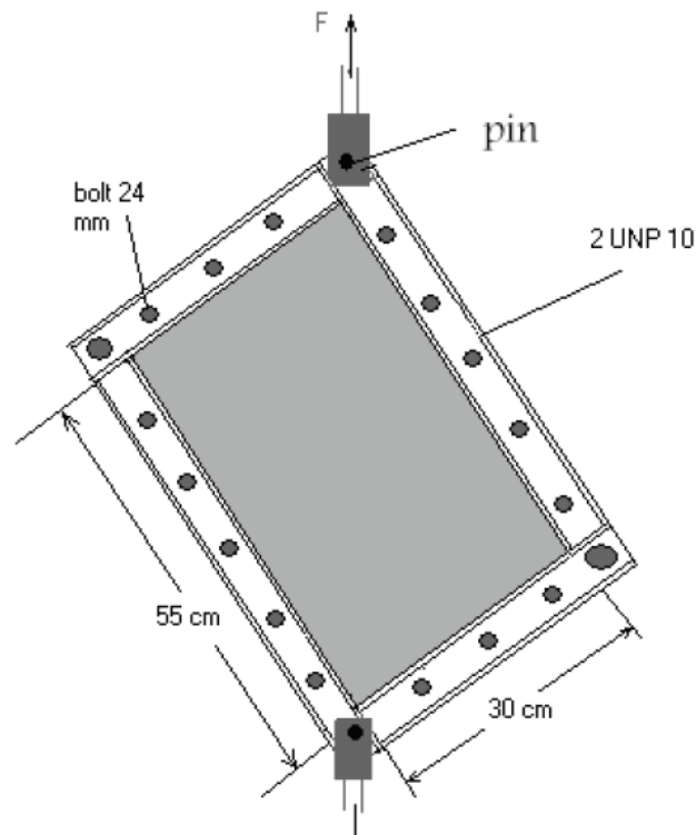
FIGURE 2-10 Test Setup (Jalali and Sazgari 2006)
