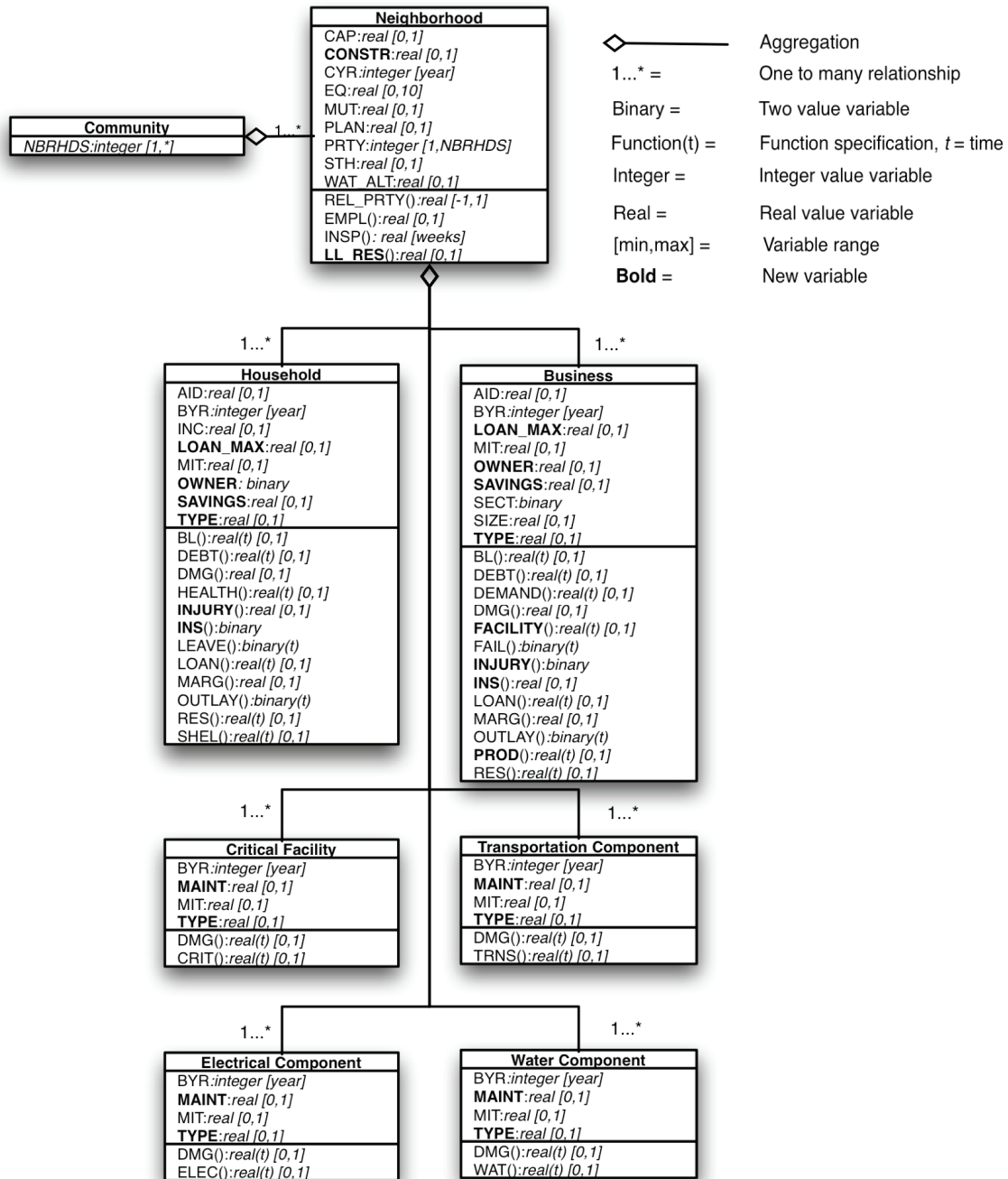
Figure 2-2 Detailed static model of community recovery from disasters.
