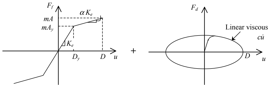
Bilinear Elastic Frame
