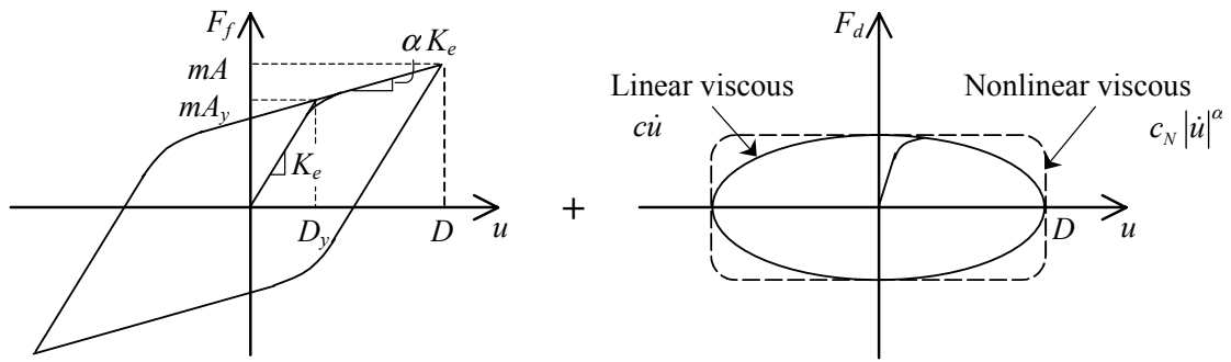
Bilinear Hysteretic Frame
