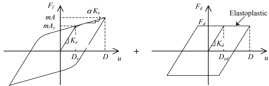
Bilinear Hysteretic Frame
