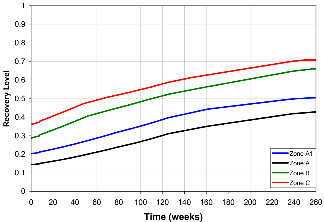
Figure 7-8. Simulated restoration of buildings by zone for Kobe using simulation prototype.
