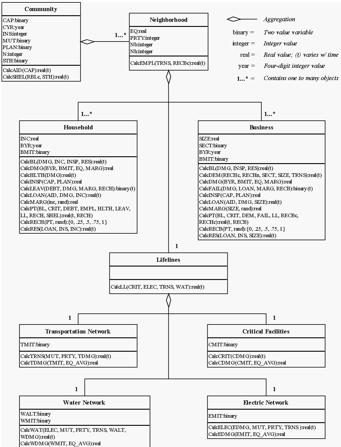
Figure 4-1. Main objects in conceptual model. The three parts of each box respectively indicate the object's name, attributes, and behaviors or functions.
