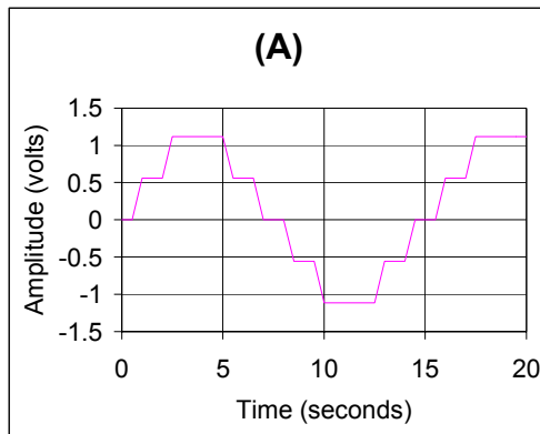
Figure 1. Sampled Sinusoidal Waveform.
